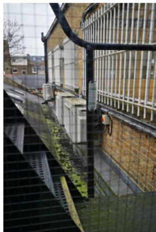
Unit 1, 2 & 3 3no. existing condenser units on second floor wall to be removed
