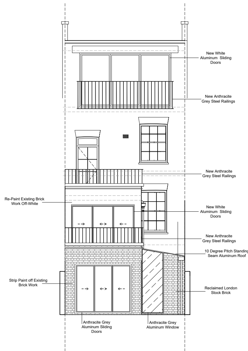
Rear Elevation
