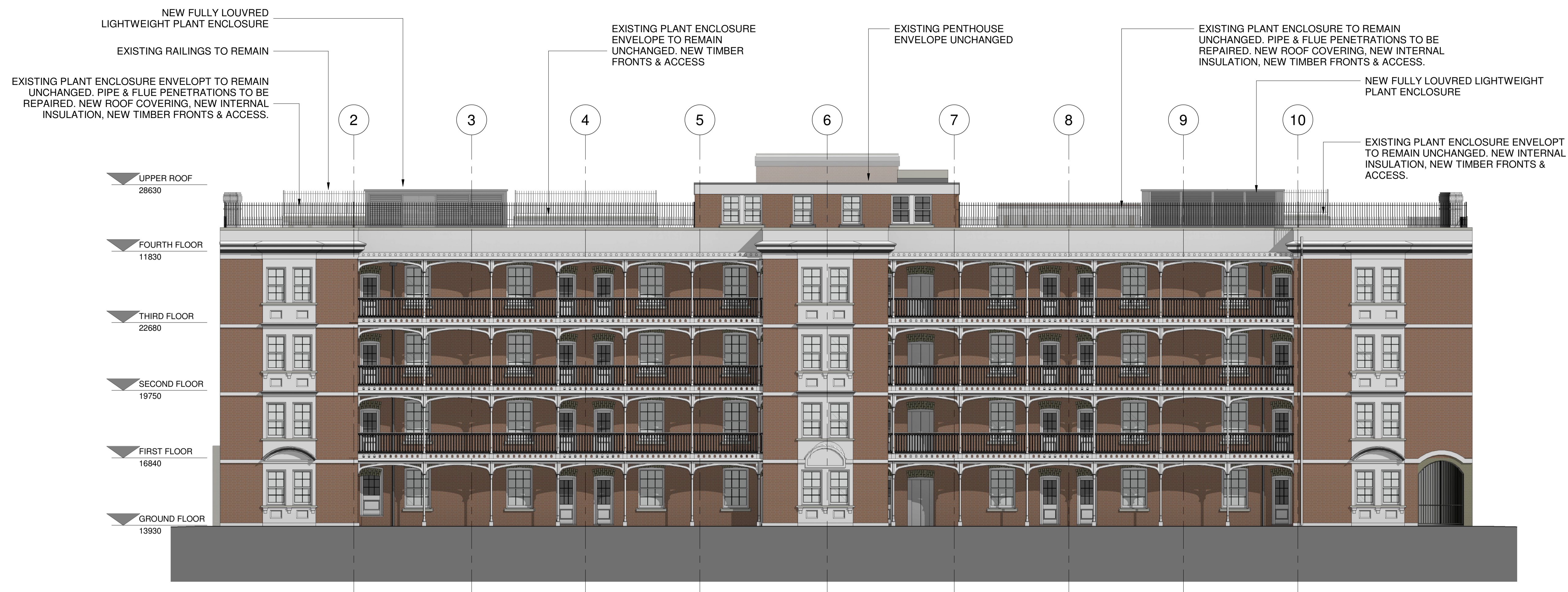
1 1 PROPOSED - EAST ELEVATION 07110 07100 1 : 100
