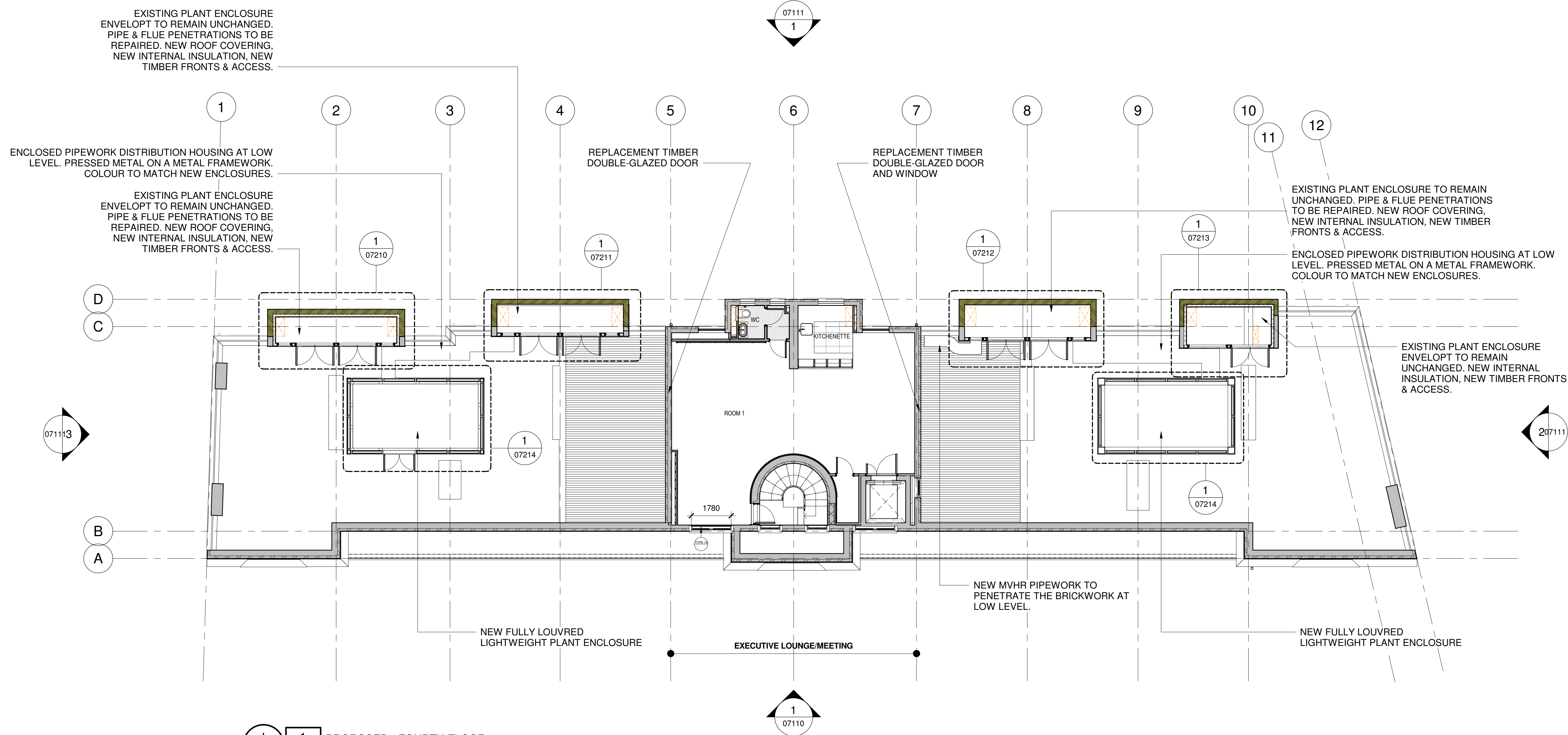
1 07104 1 01110 PROPOSED - FOURTH FLOOR 1:100
