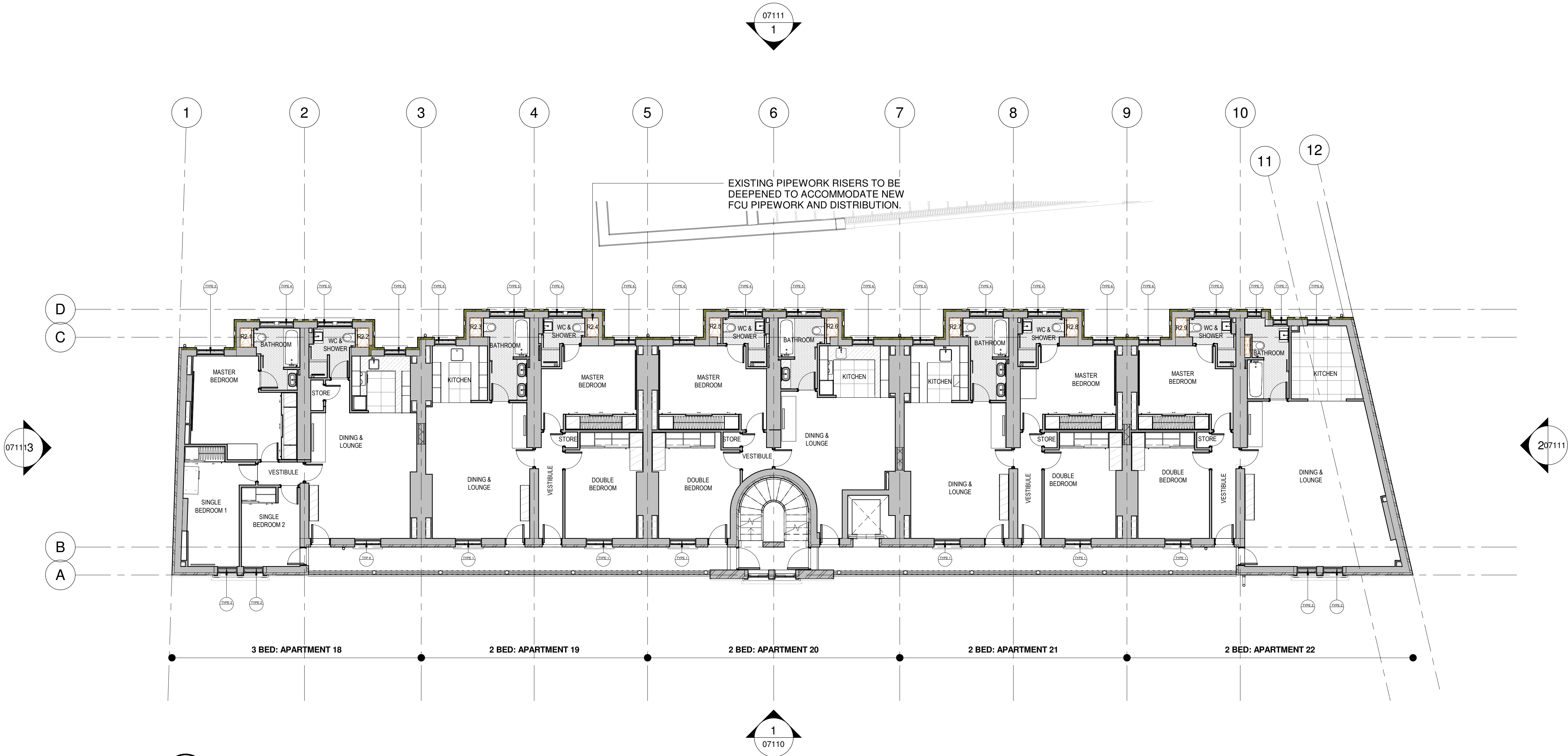
1 1 PROPOSED - SECOND FLOOR 07102 01110 1:100
