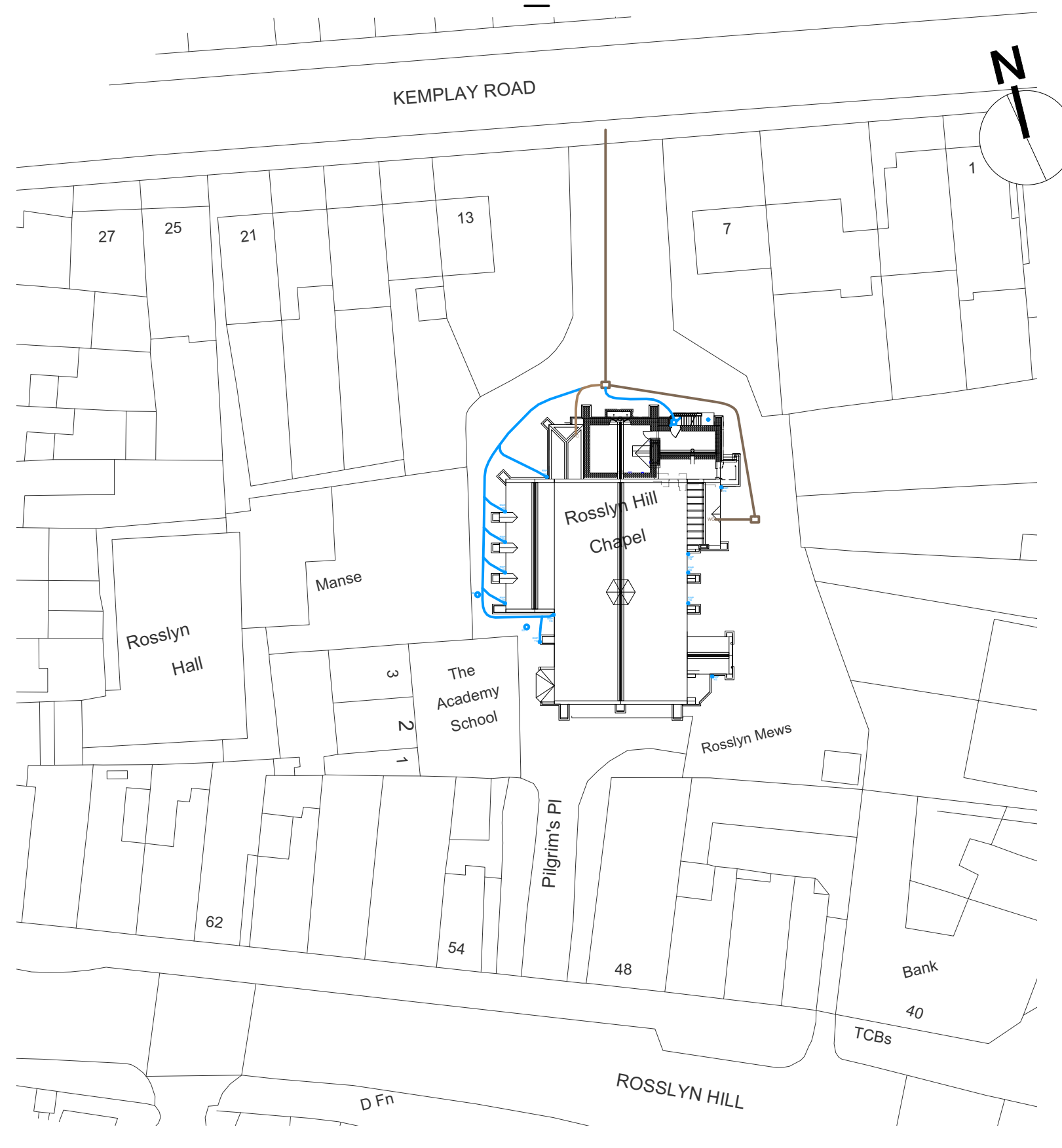
BLOCK PLAN SHOWING CRYPT LOCATION AND SCHEMATIC DRAINAGE Scale: 1:500
