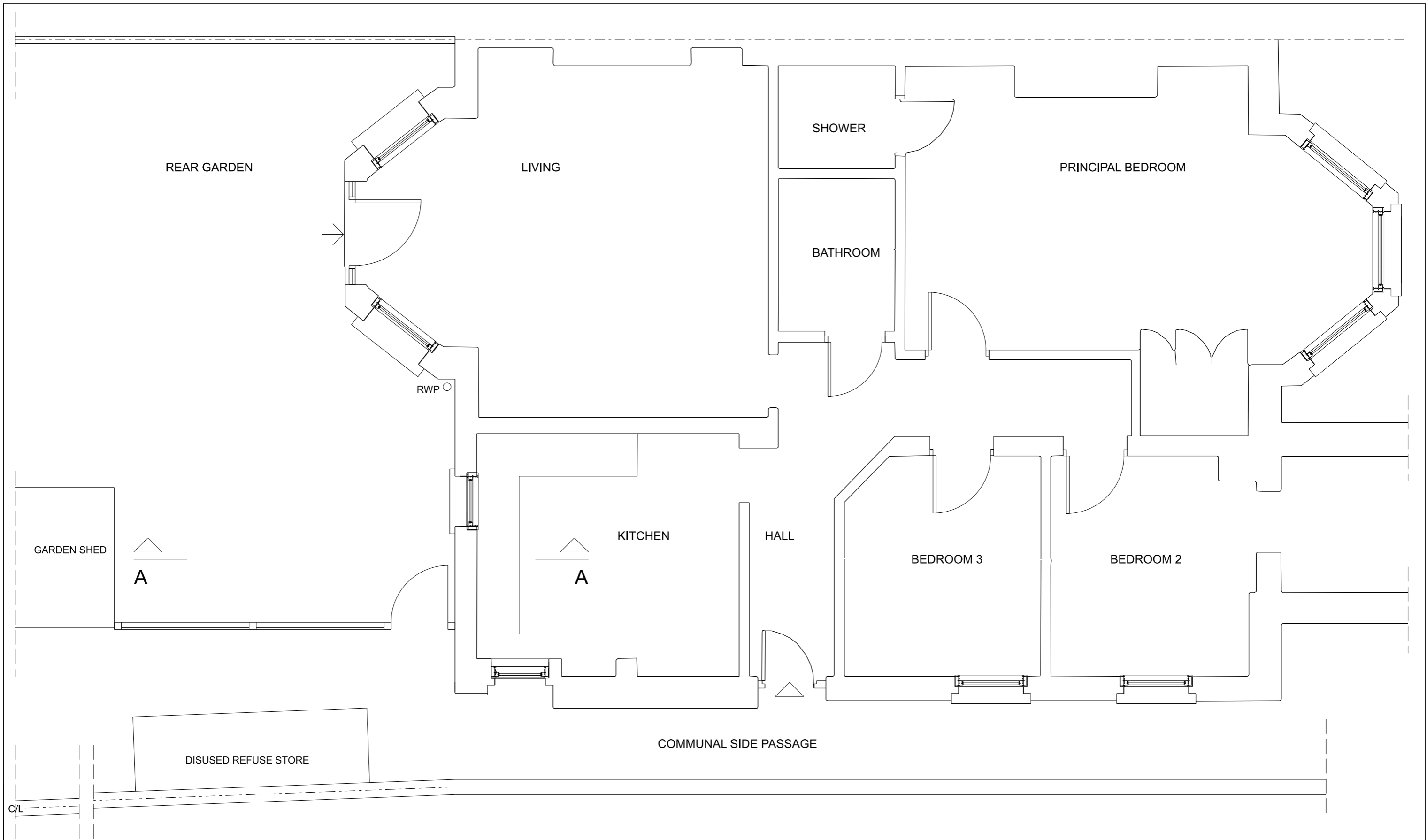
03 LOWER GROUND FLOOR PLAN AS EXISTING A
