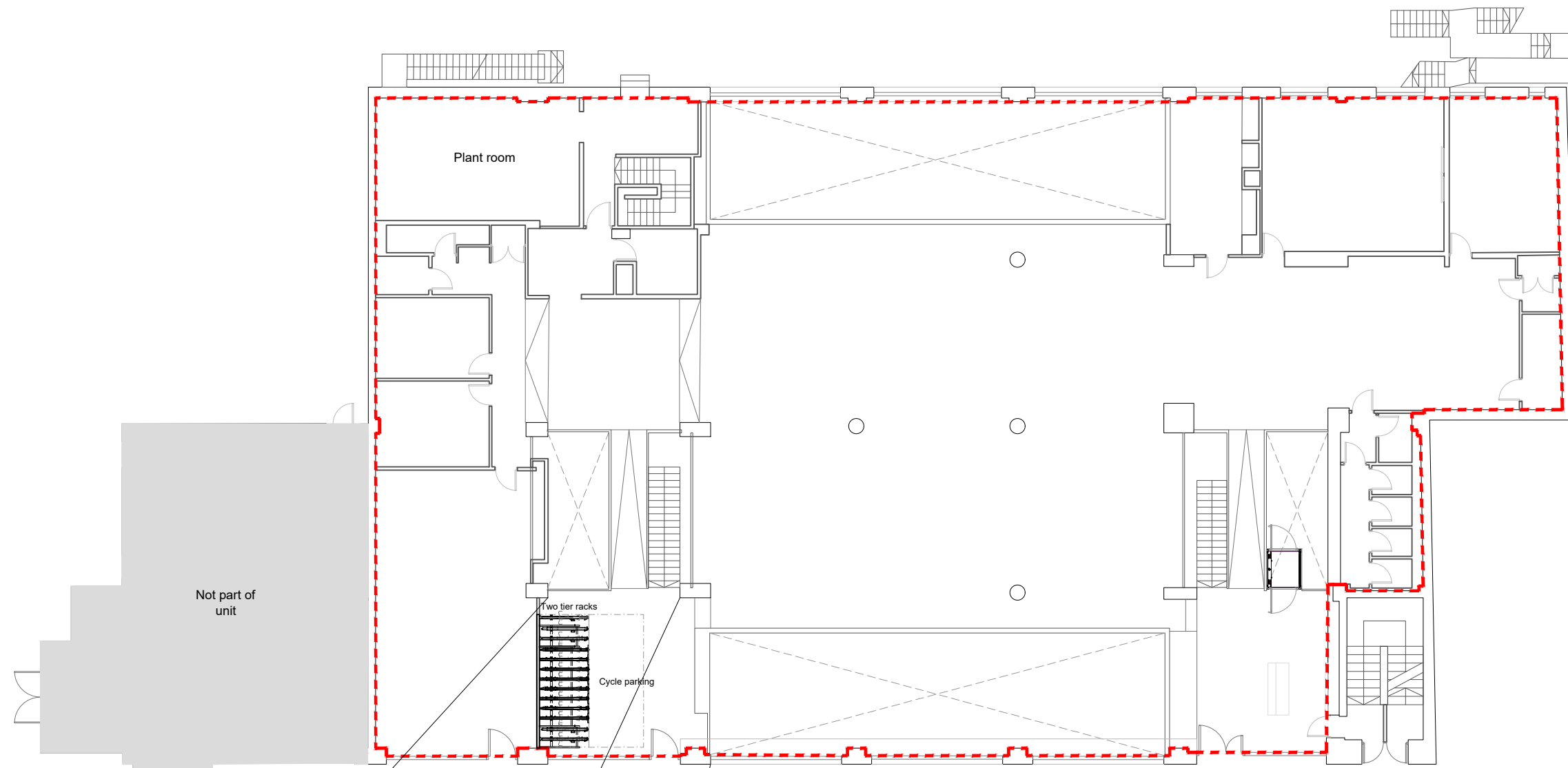
Proposed Ground floor 1:200
