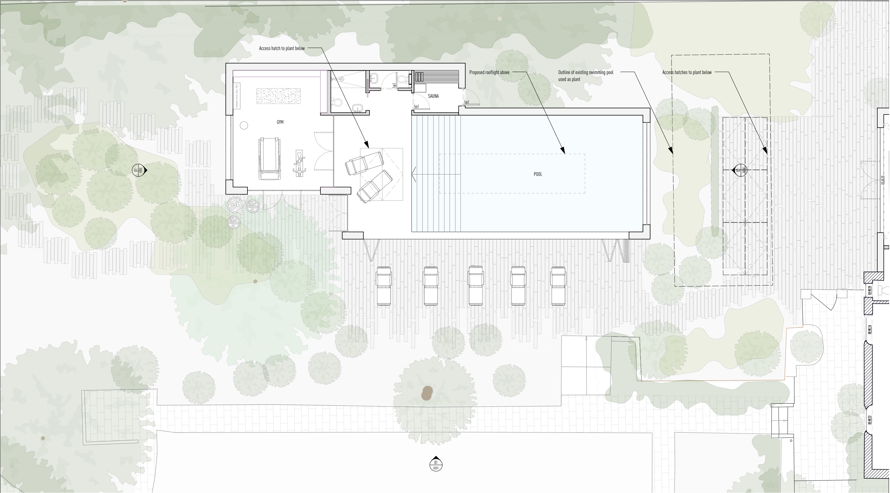
01 - Proposed Ground Floor Plan 1:100 @ A3
