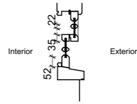
3 Existing Window Section 1:20
