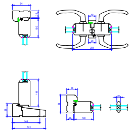
2 Proposed Door Details 1:20
