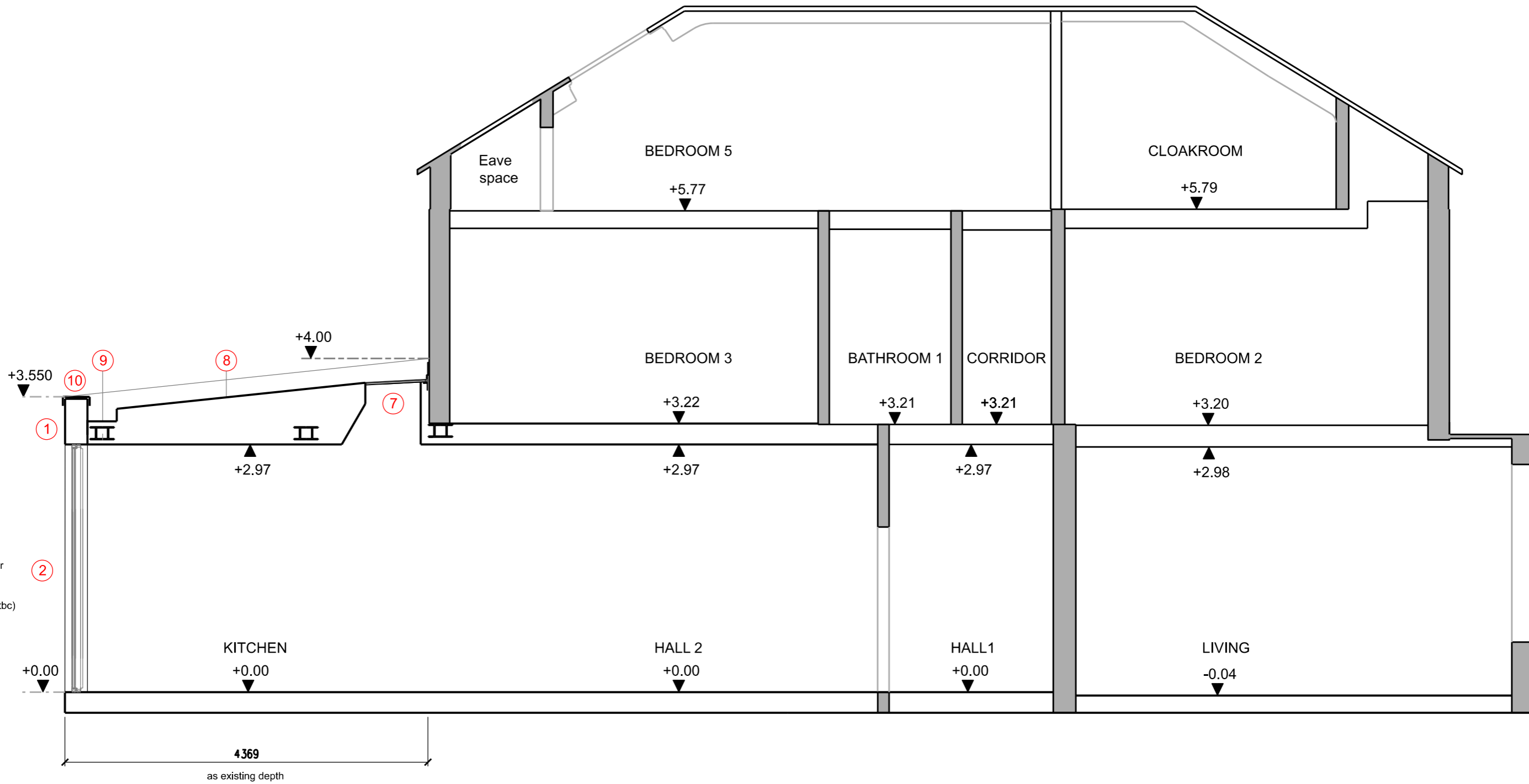
1 PROPOSED LONGITUDINAL SECTION A-A
