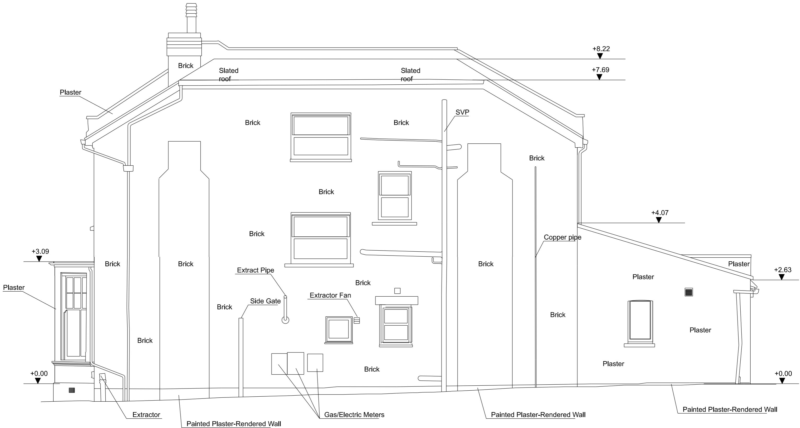
1 EXISTING SIDE ELEVATION
