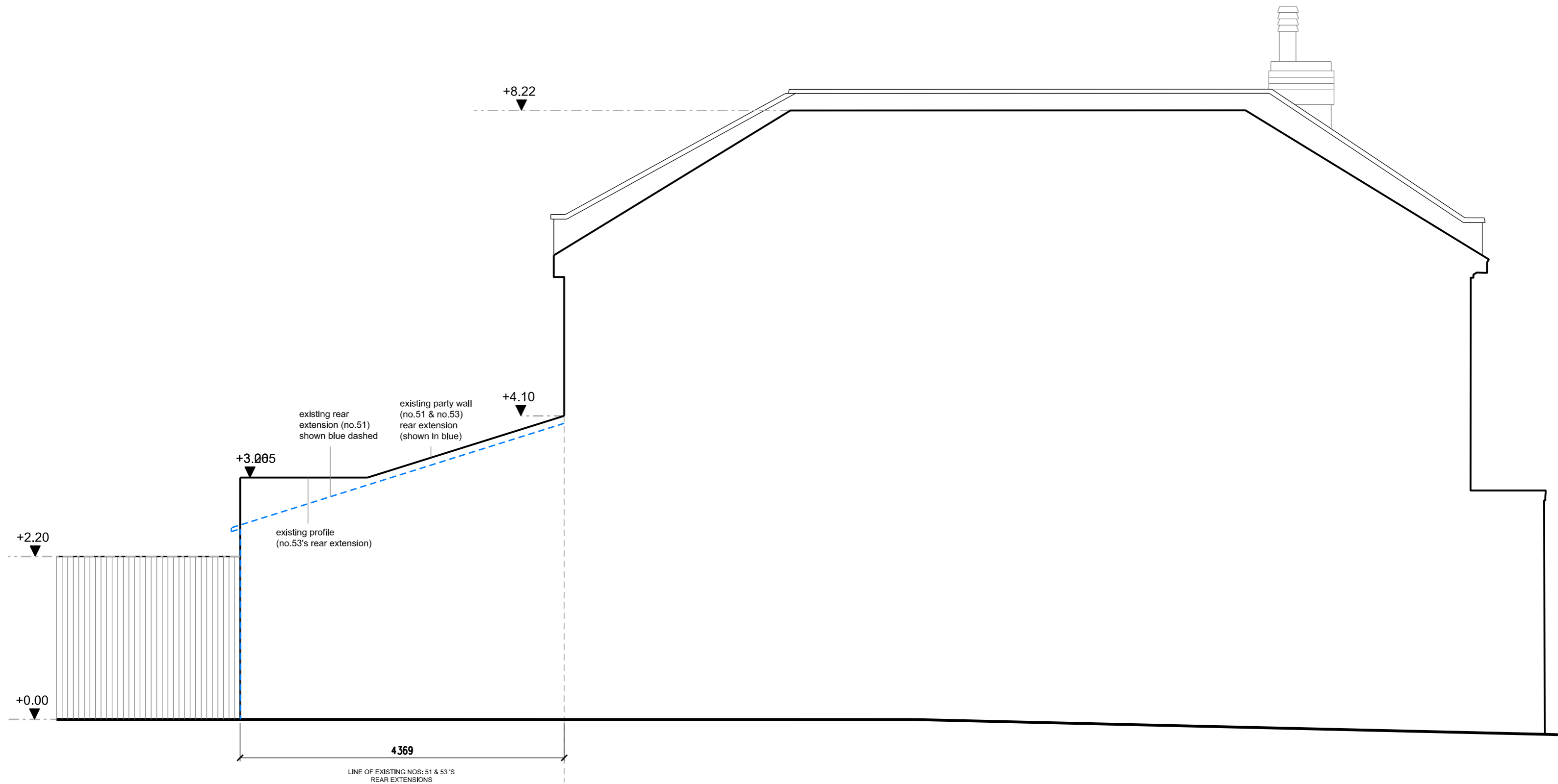
1 EXISTING SIDE ELEVATION 2 ADJOINING NO.53
