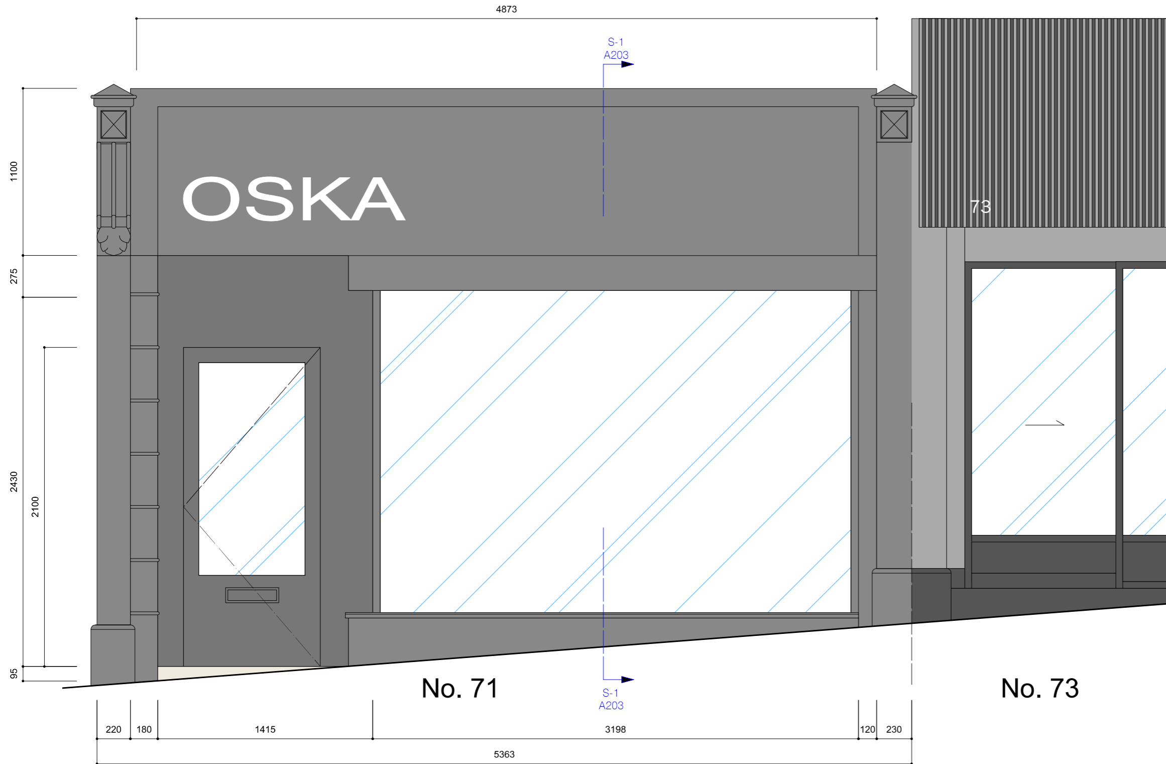
Shopfront elevation S=1/25@A3
