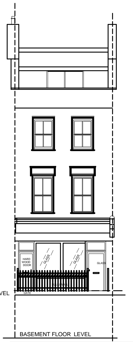
FRONT ELEVATION AS EXISTING
