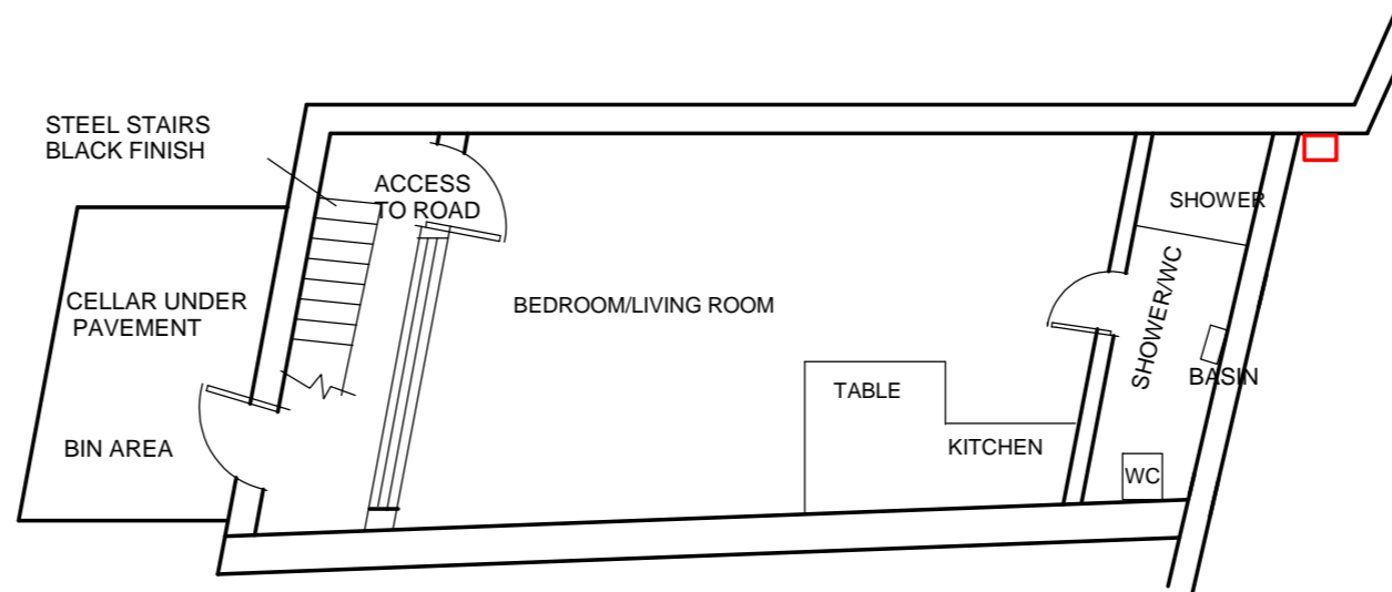
BASEMENT FLOOR PLAN AS EXISTING
