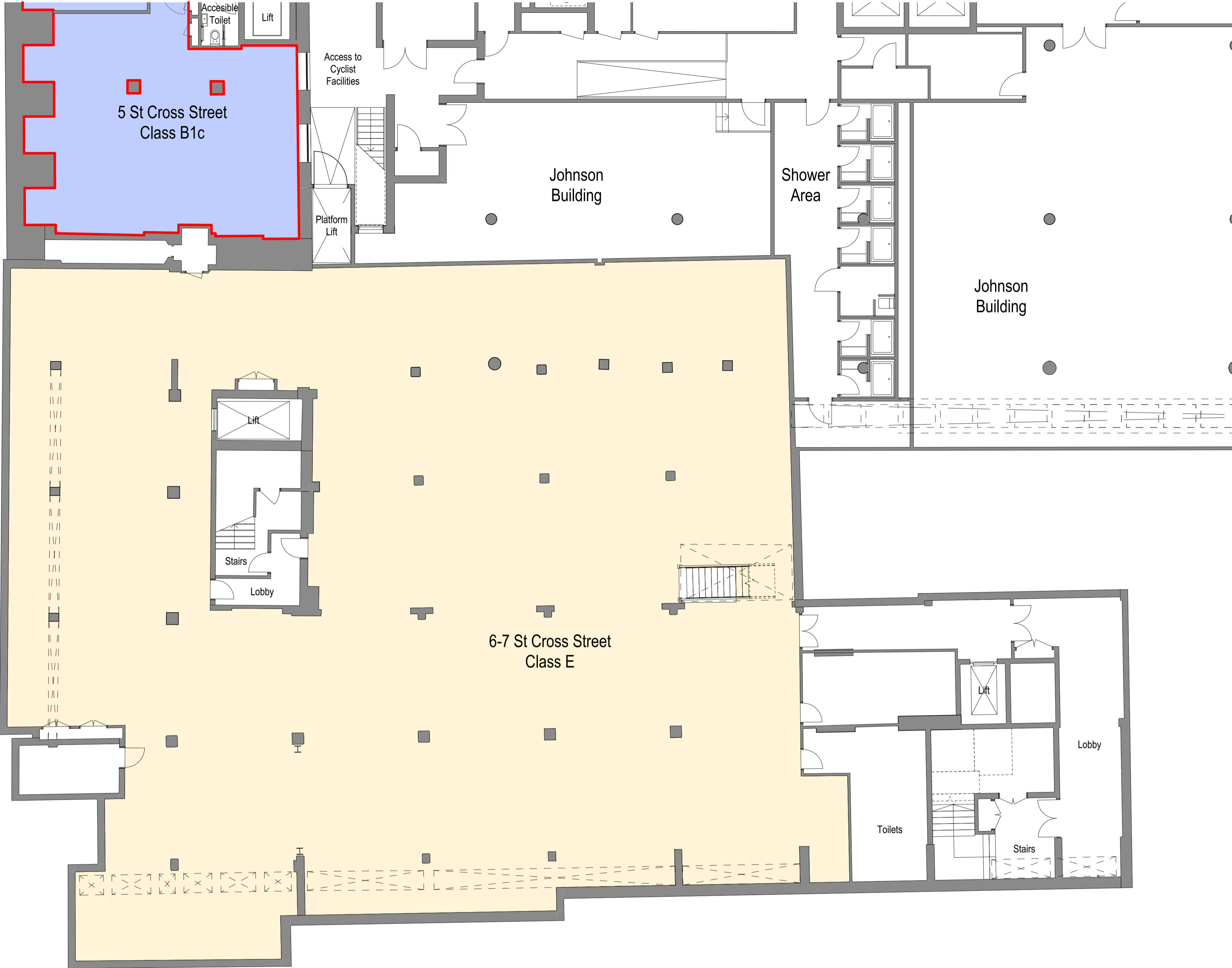
1 6-7 St Cross Street - Existing Lower Ground Floor SCALE 1:100
