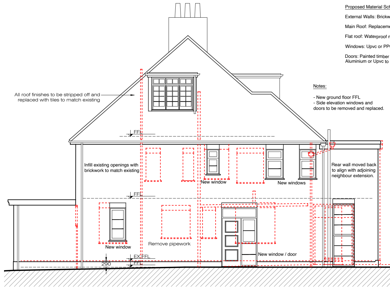
SIDE ELEVATION
