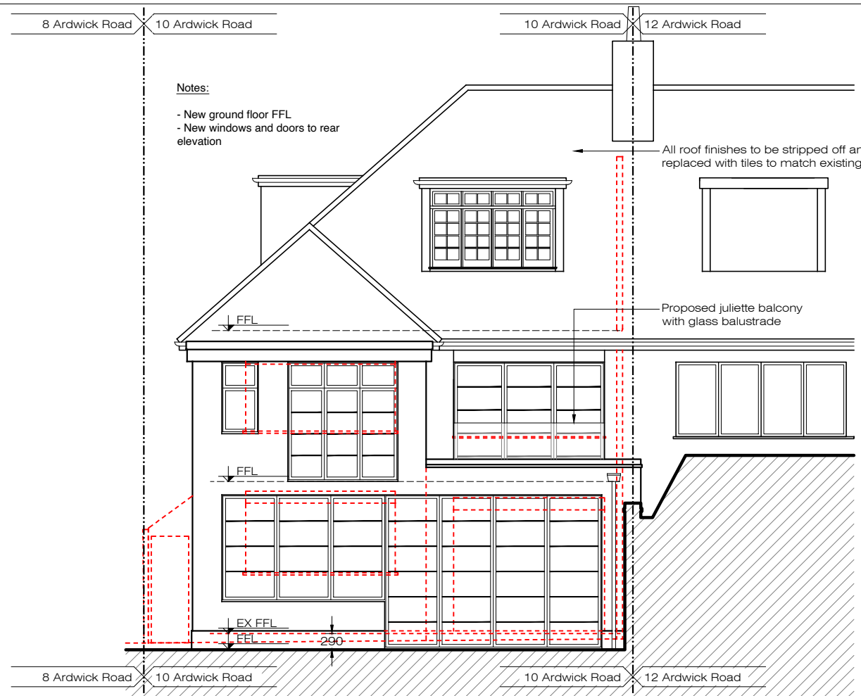
REAR ELEVATION
