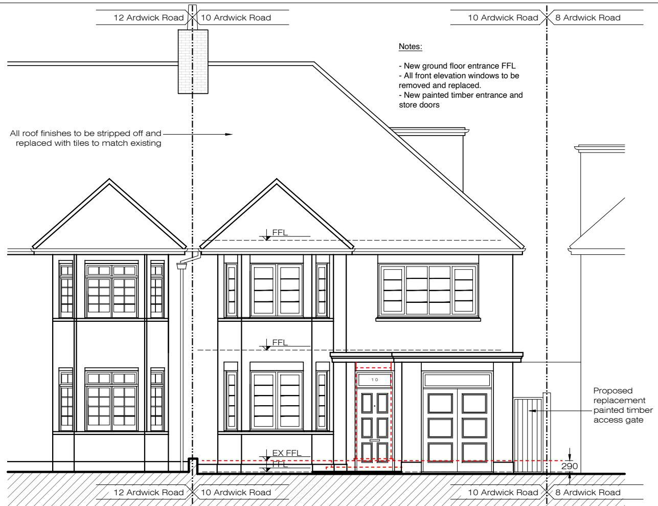
FRONT ELEVATION
