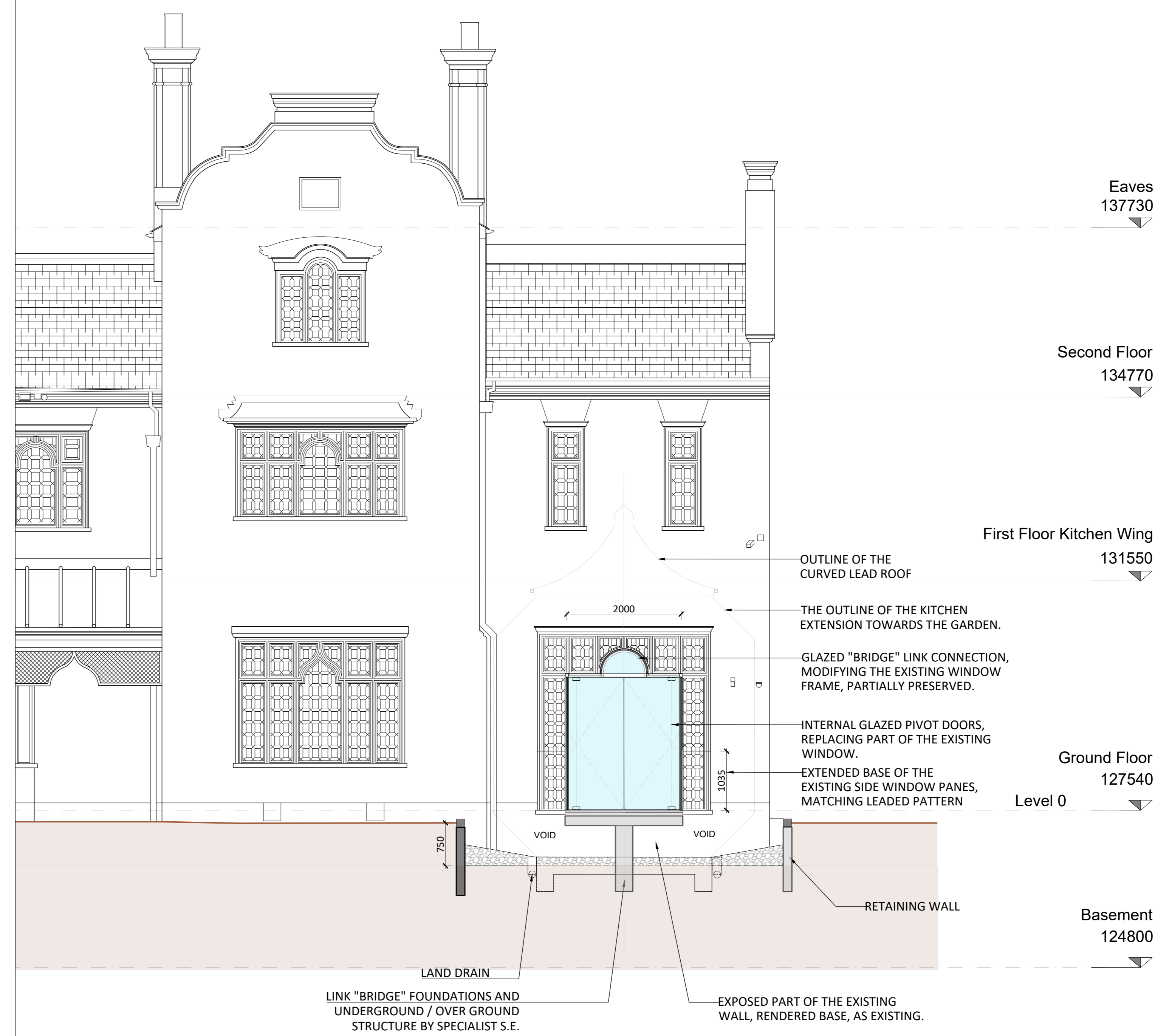
SECTION E-E
