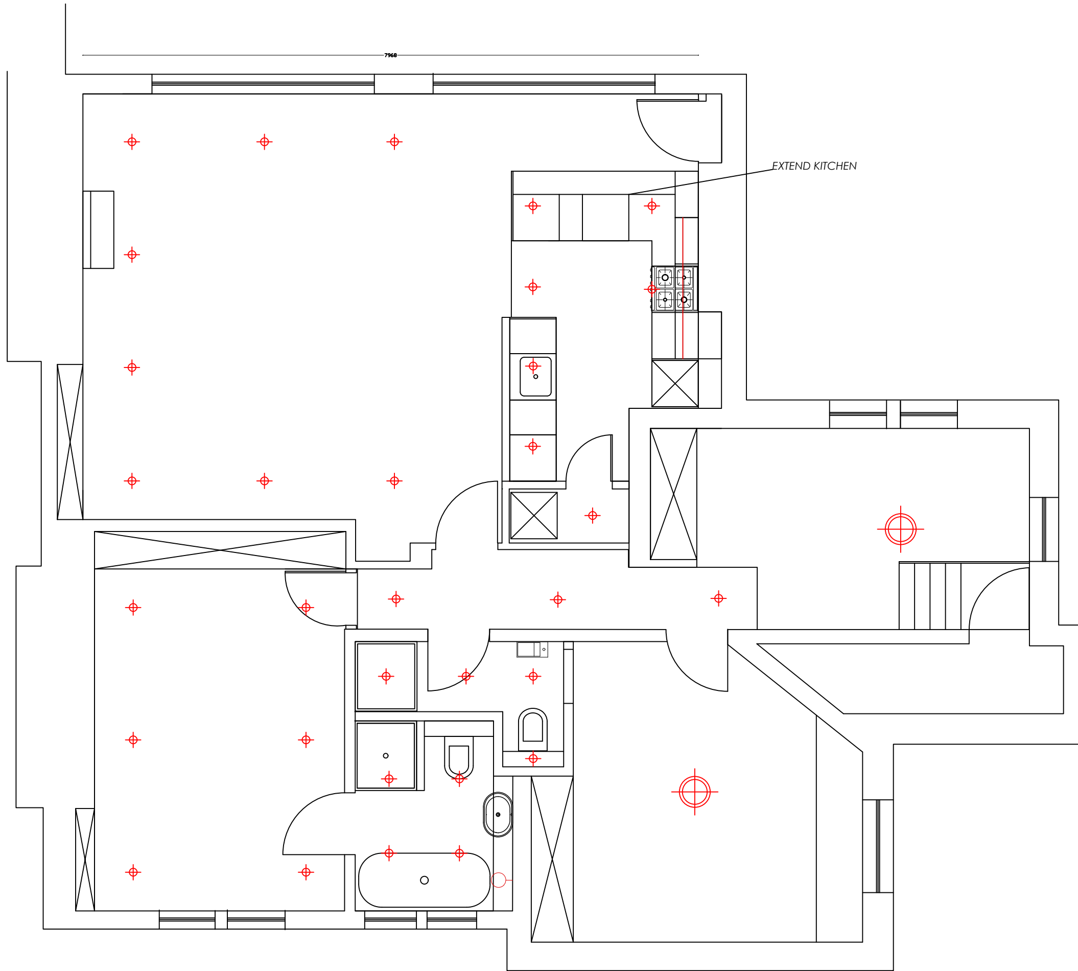
PROPOSED LIGHTING LAYOUT
