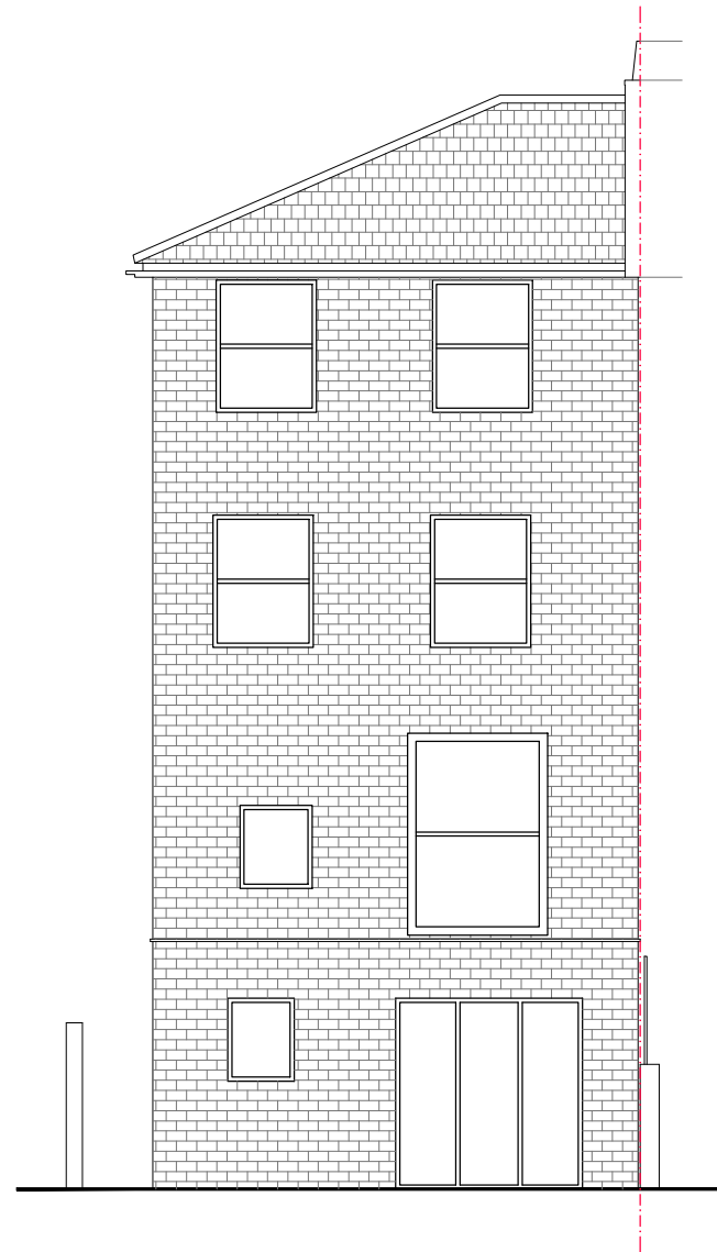
EXISTING REAR ELEVATION (Remains as existing)
