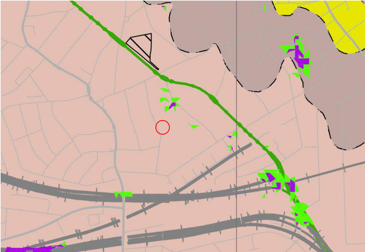
Figure 10 Slope Angle and Worked Ground Map, LB Camden (GHHS figure 16)
