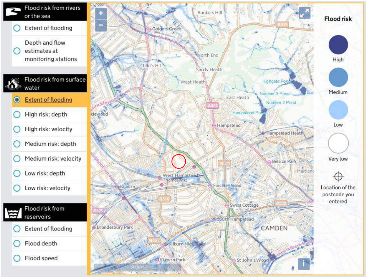
Figure 13 Flood Risk Map, Environment Agency (Surface Water Flood Risk)
