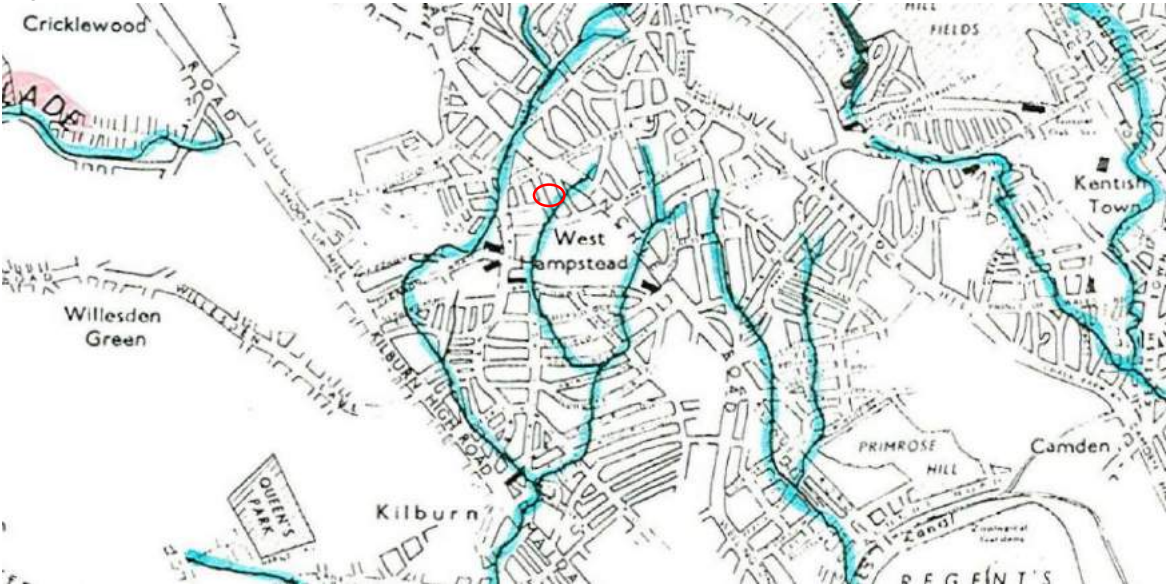
Figure 15 Lost Rivers of London, Barton (LB Camden GHHS Figure 11)
