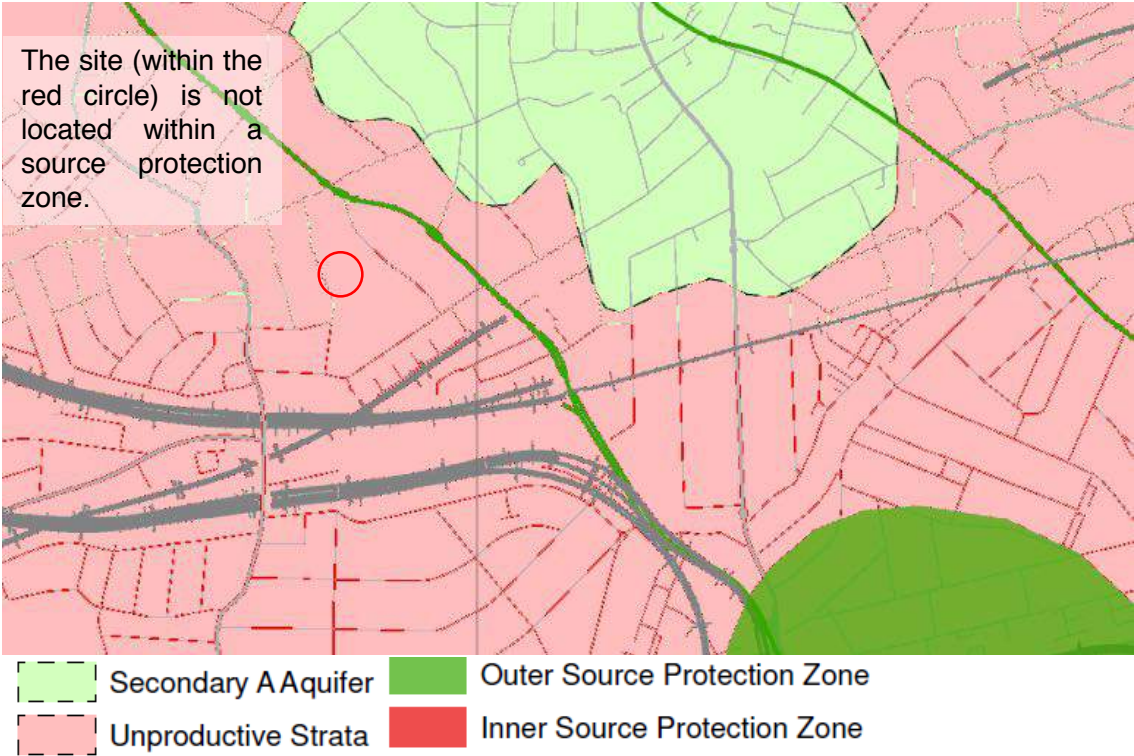
Figure 14 Groundwater Source Protection Zone, LB Camden (GHHS Figure 8)
