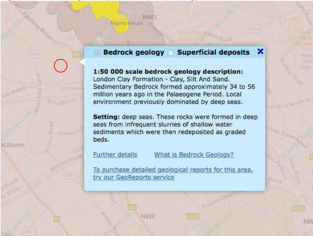
Figure 11 Geological Map Extract, BGS (Geology of Britain Viewer)
