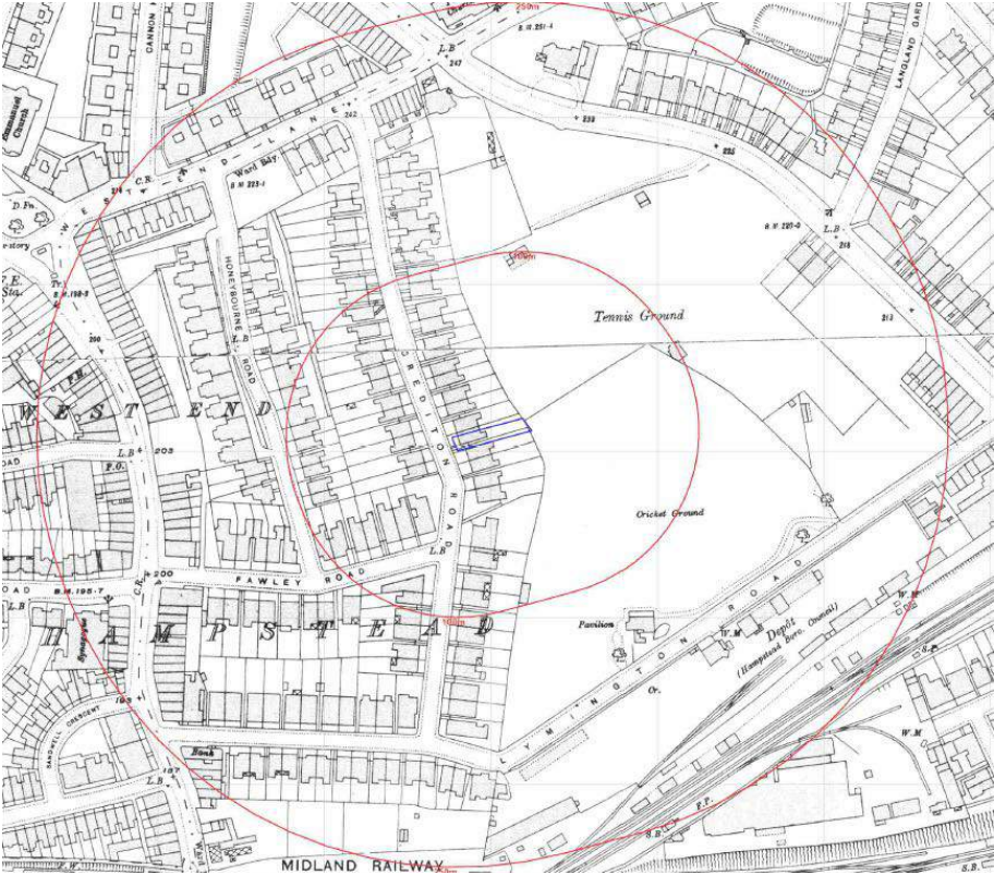
Figure 6 Historical Map Extract, OS 1:2,500 1915
