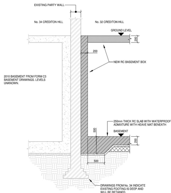
Figure 10: Proposed section to party wall
