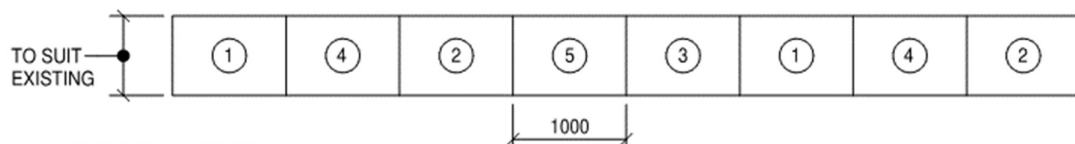
Figure 9- Indicative Underpinning Sequence
