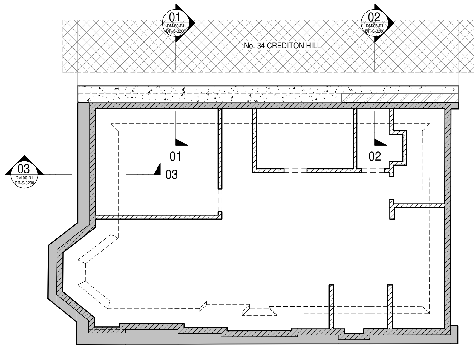
BASEMENT KEY PLAN
