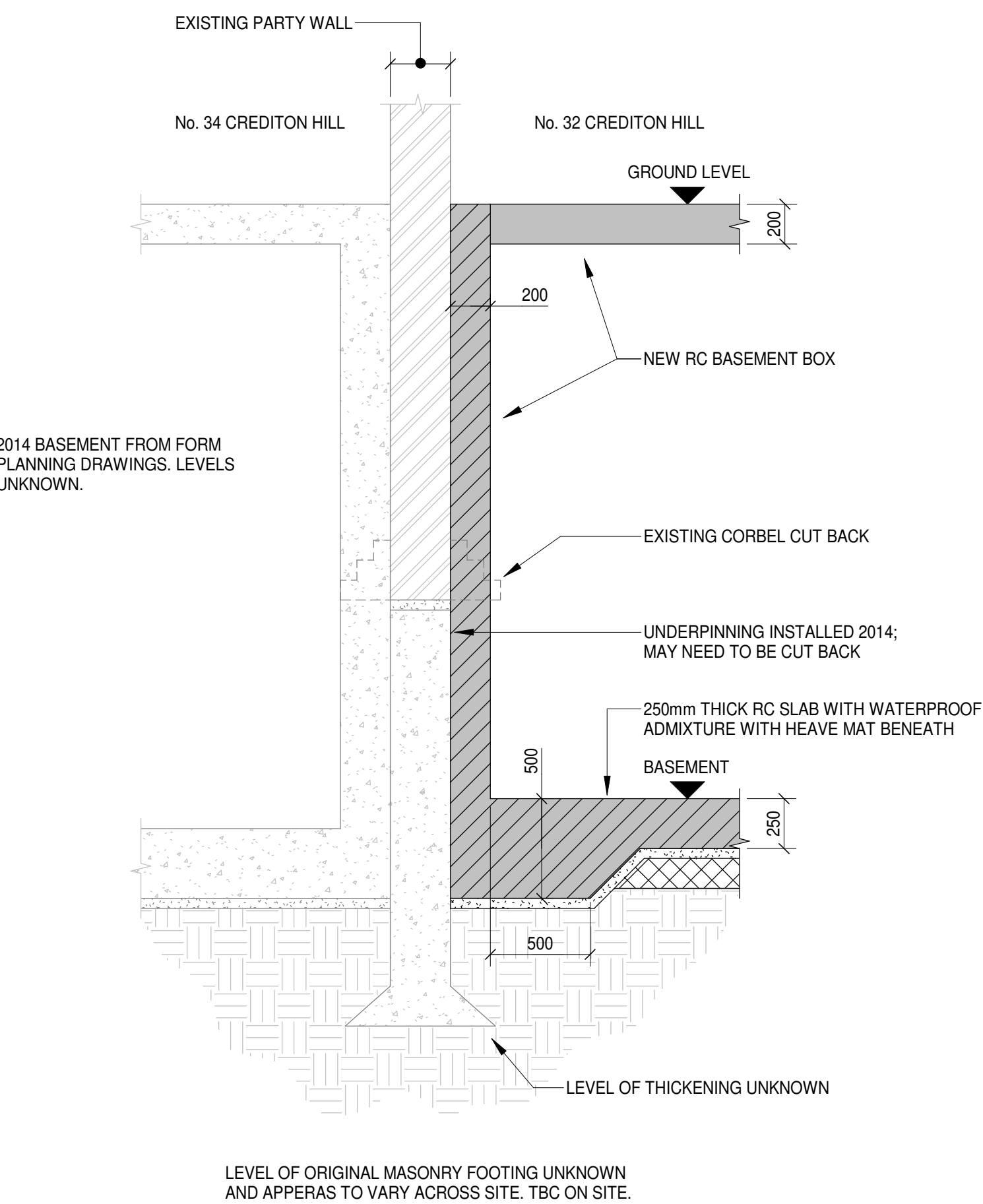
BASEMENT SECTION
