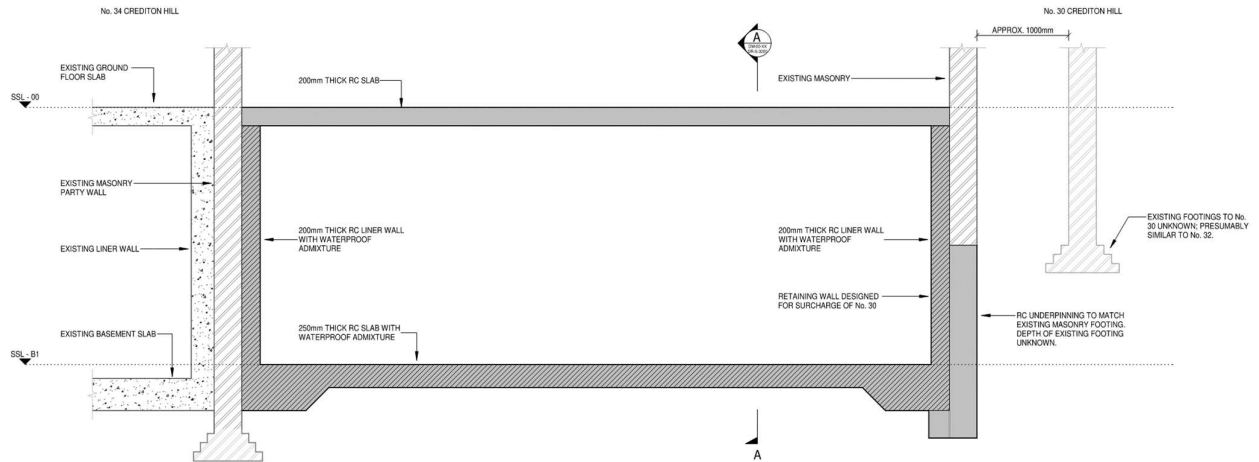
Figure 9: Section showing neighbouring building foundations
