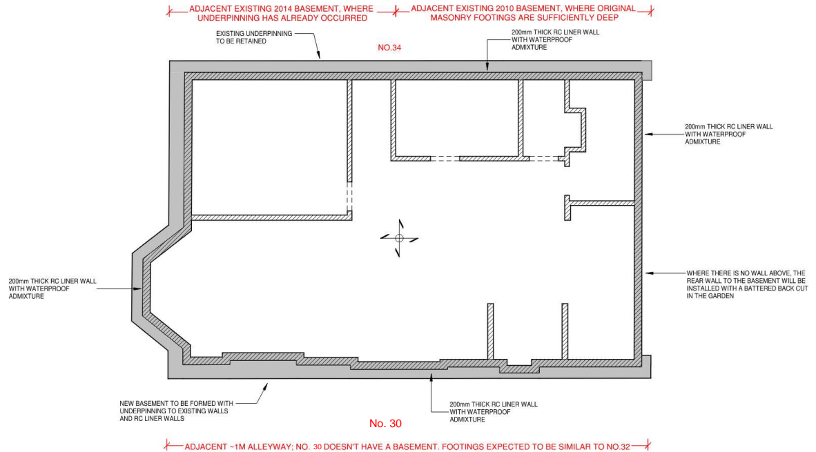
Figure 8- Proposed Basement Floor Plan
