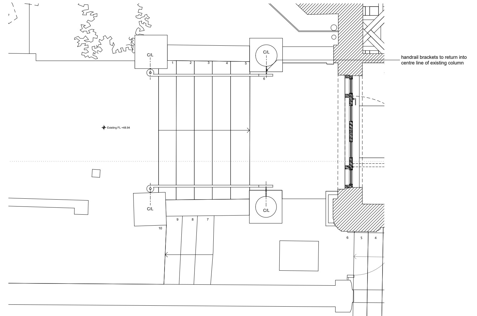
02 Plan view - Proposed handrail and guarding 2902 Scale: 1:20 (A1), 1:40 (A3)
