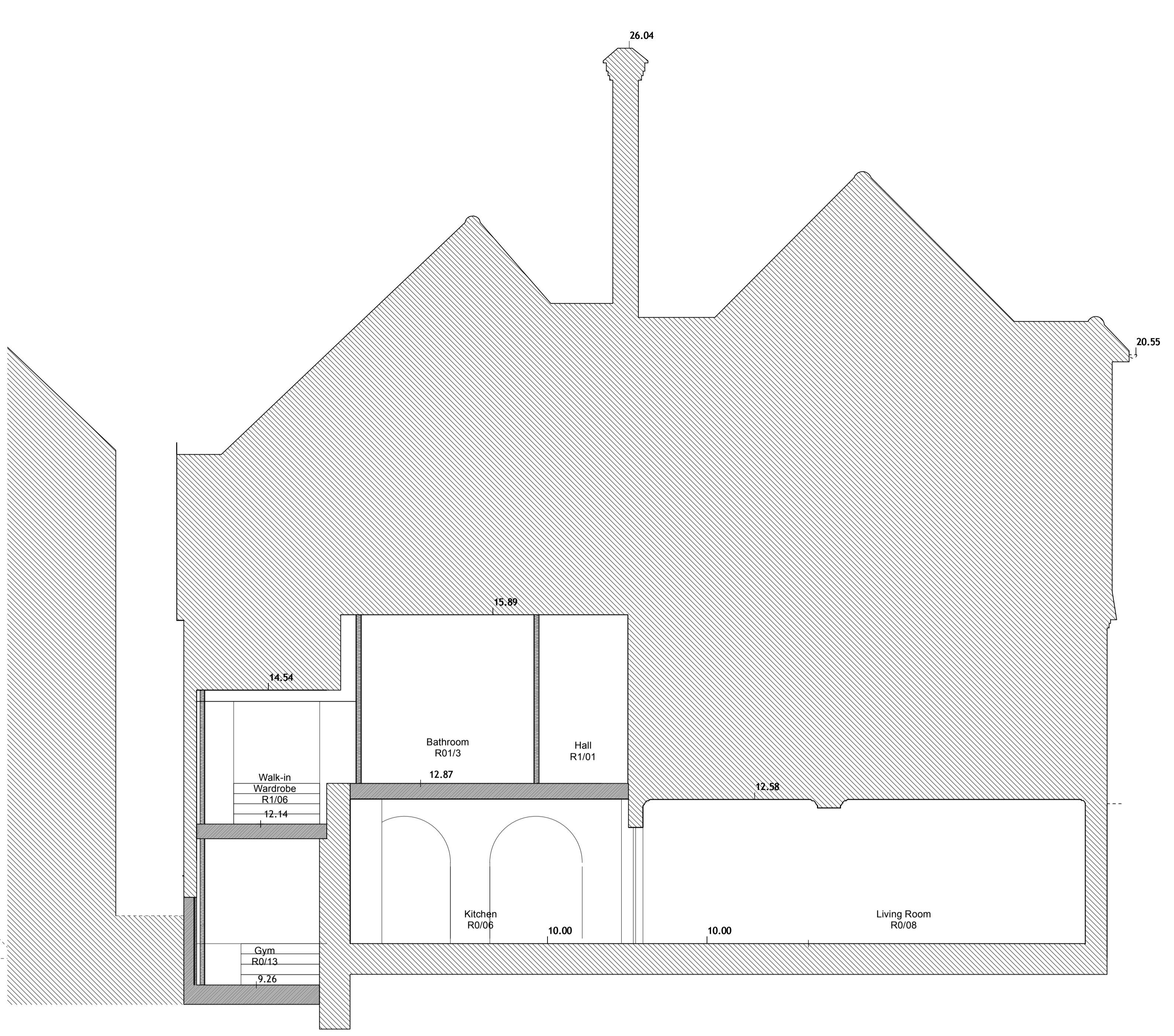
2 Proposed Section C-C Scale: 1:50
