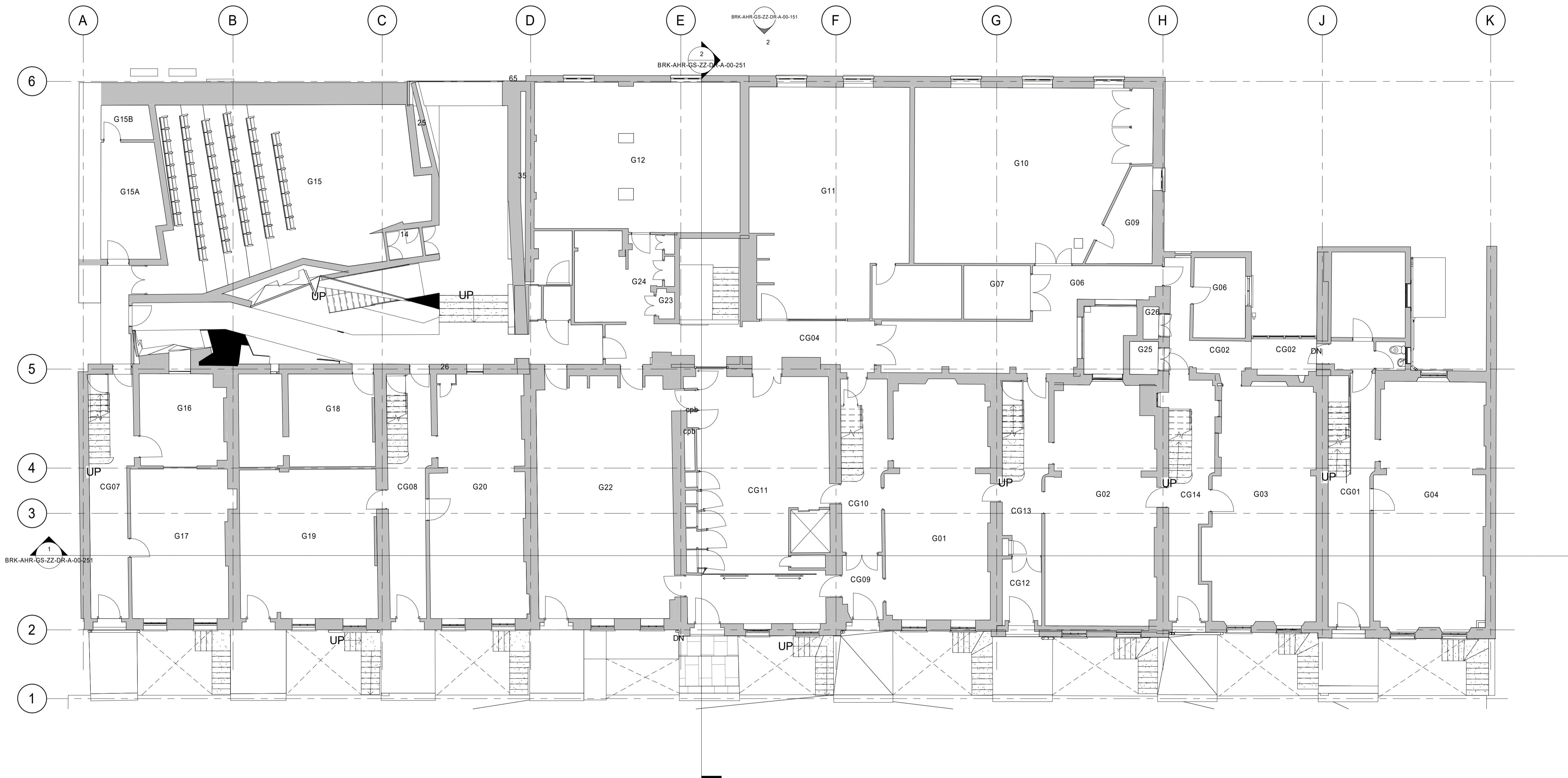
1. Planning - LEVEL 00 - Existing 1 : 100
