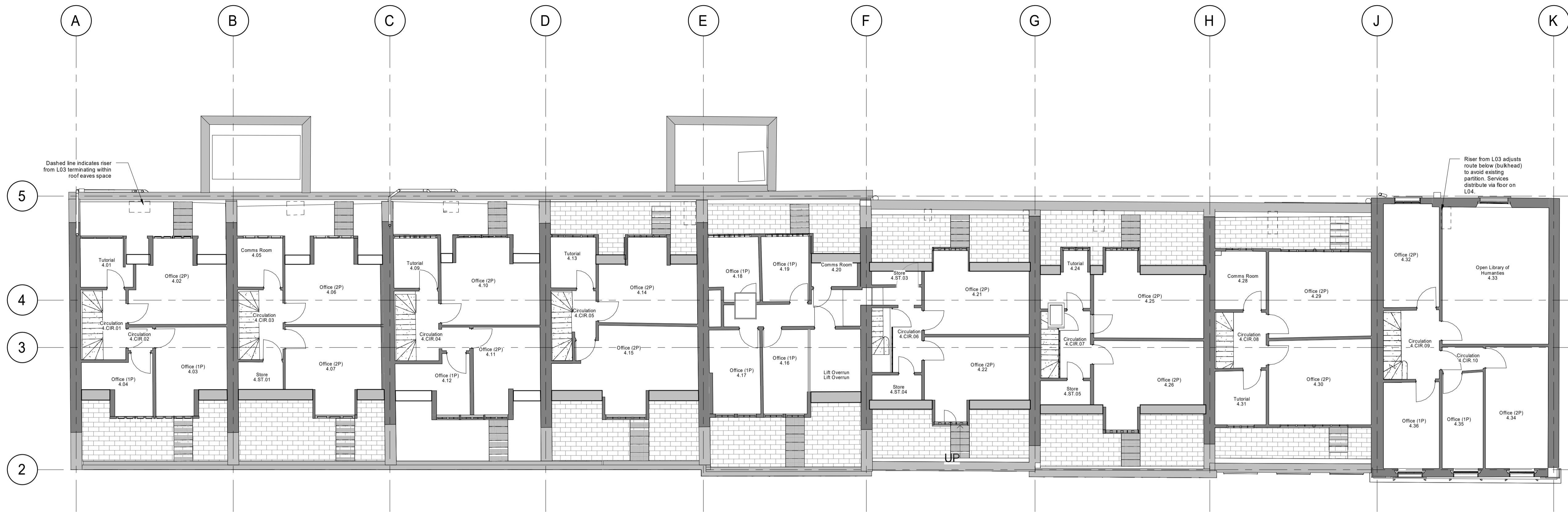
2. Planning - LEVEL 04 - Proposed Heritage Impact 1 : 100
