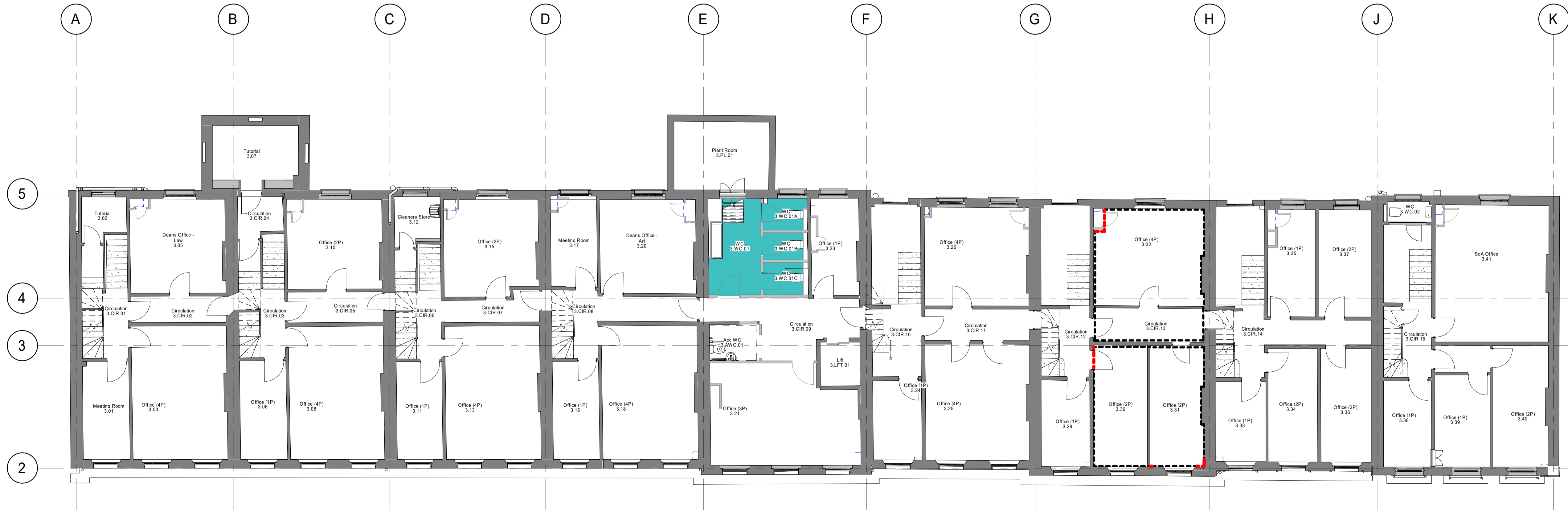
1. Planning - LEVEL 03 - Proposed Heritage Impact 1 : 100
