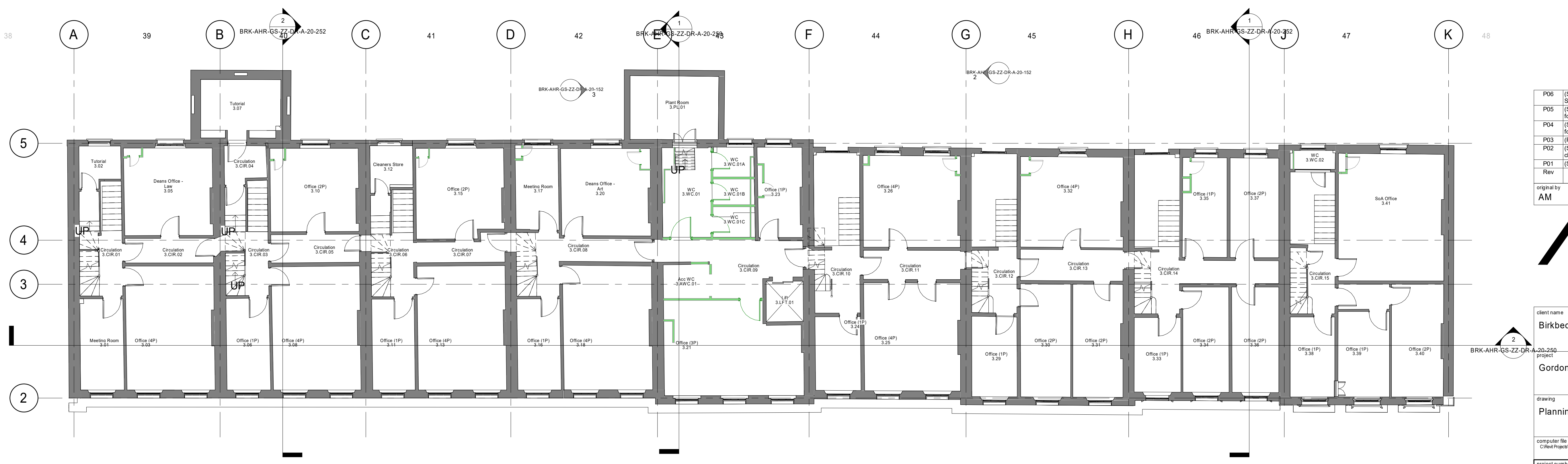
1. Planning - LEVEL 03 - Proposed 1 : 100
