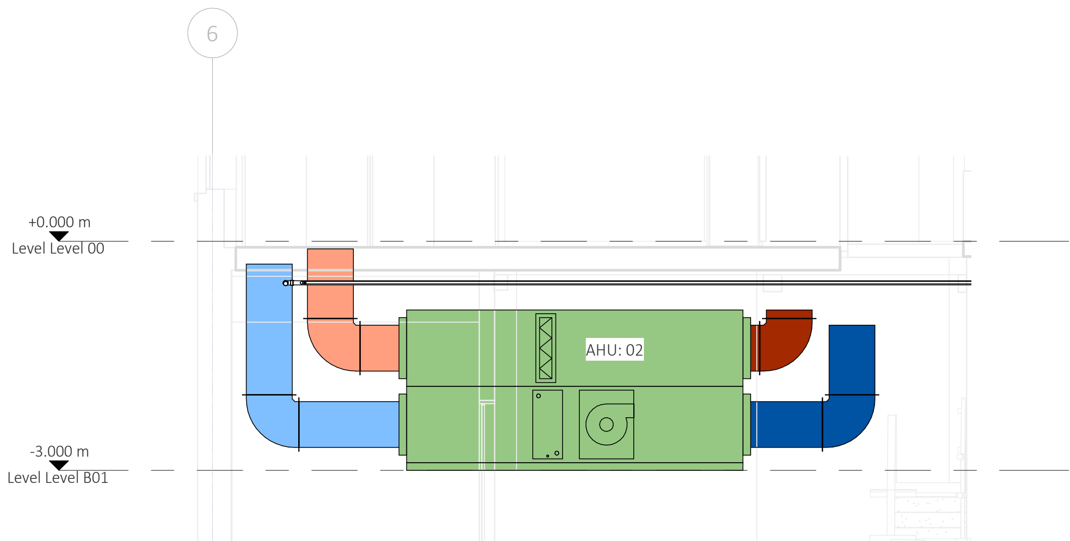
3 Lecture Theatre Ventilation Plantroom Section 1 : 50
