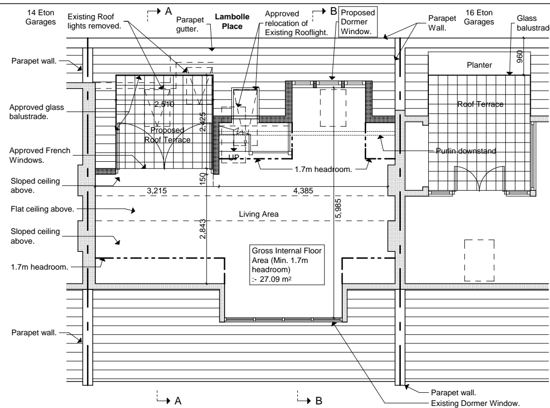
Proposed Attic Plan
