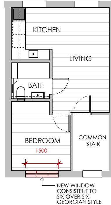
PROPOSED PLAN SCALE 1:100
