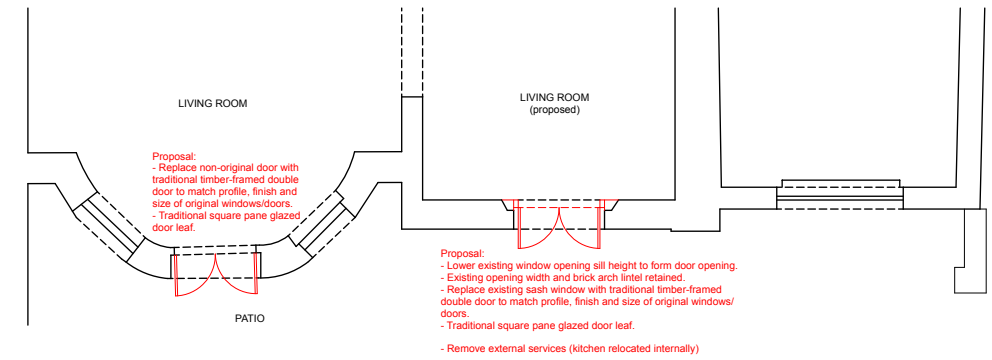
Proposed Garden Floor Plan_1:100
