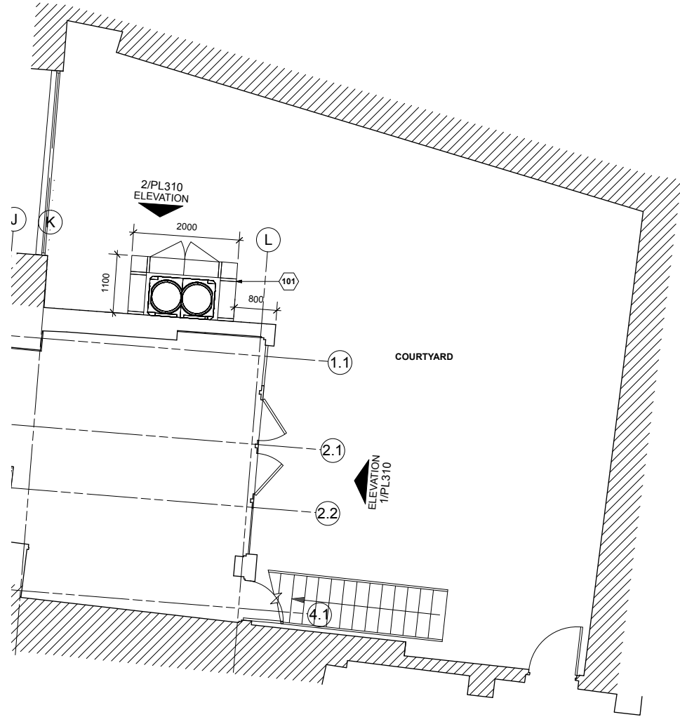
1 PROPOSED COURTYARD FLOOR PLAN PL110
