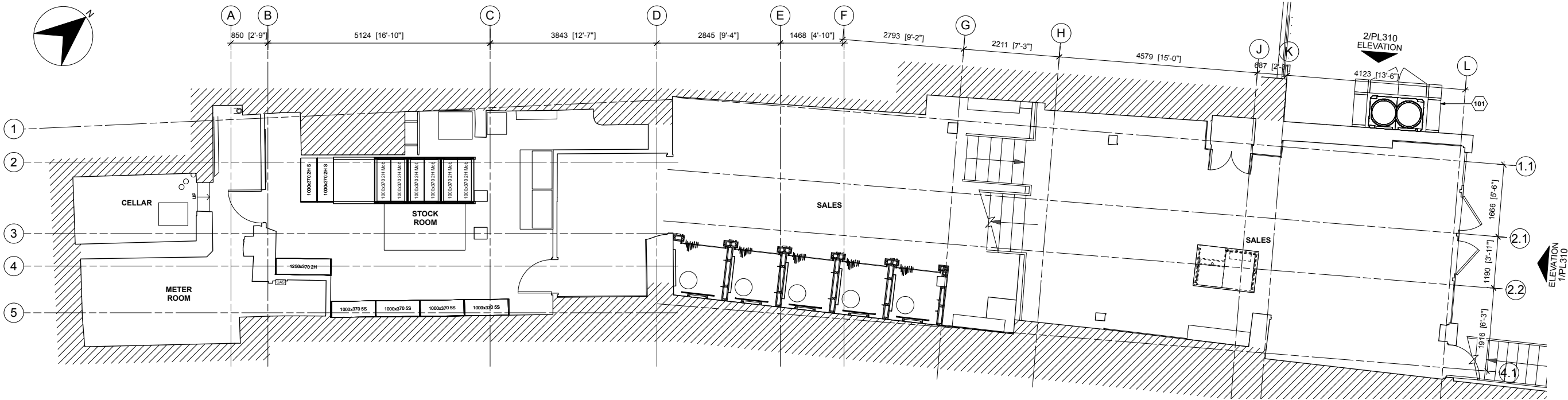
2 PROPOSED BASEMENT FLOOR PLAN PL110
