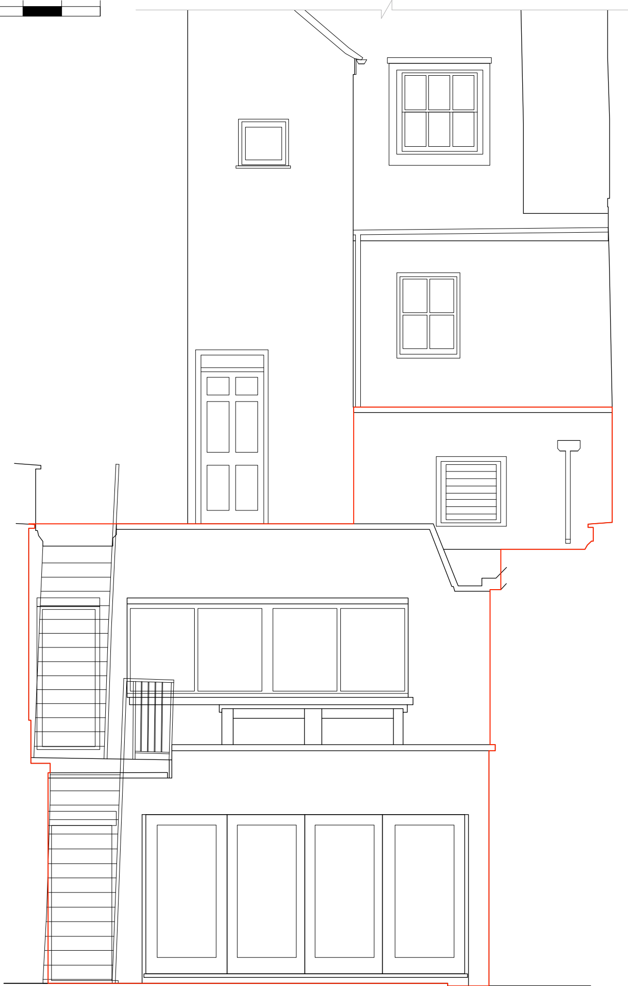
1 REAR ELEVATION EX310 SCALE: @A1 1:25
