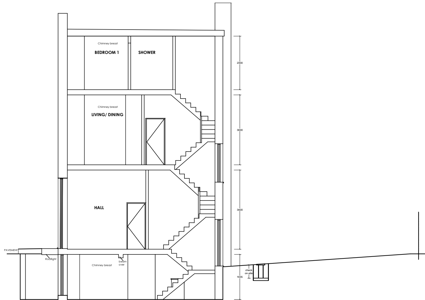
SECTION
