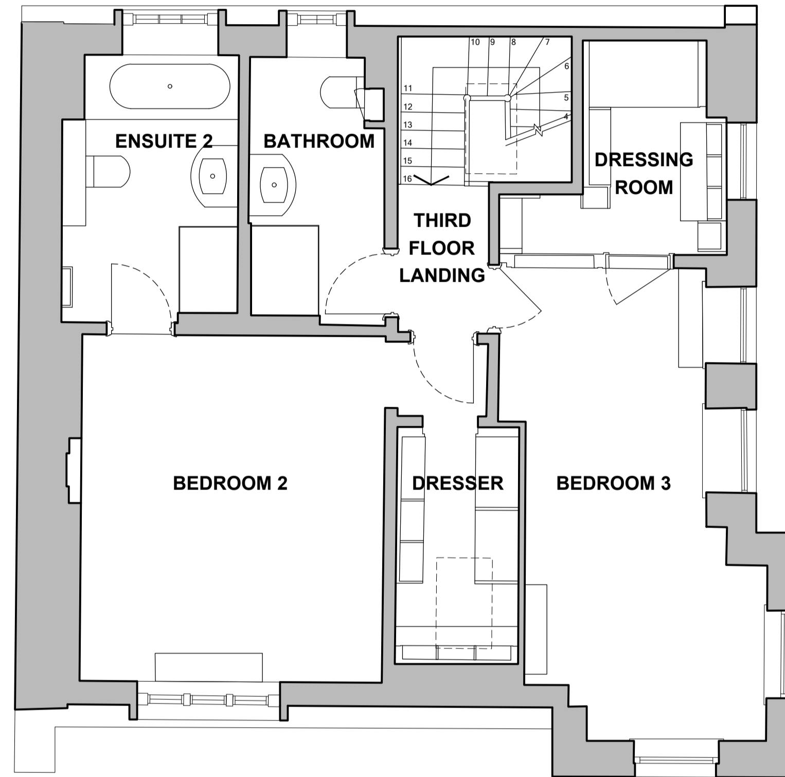
01 THIRD FLOOR PLAN 1:50 @ A1
