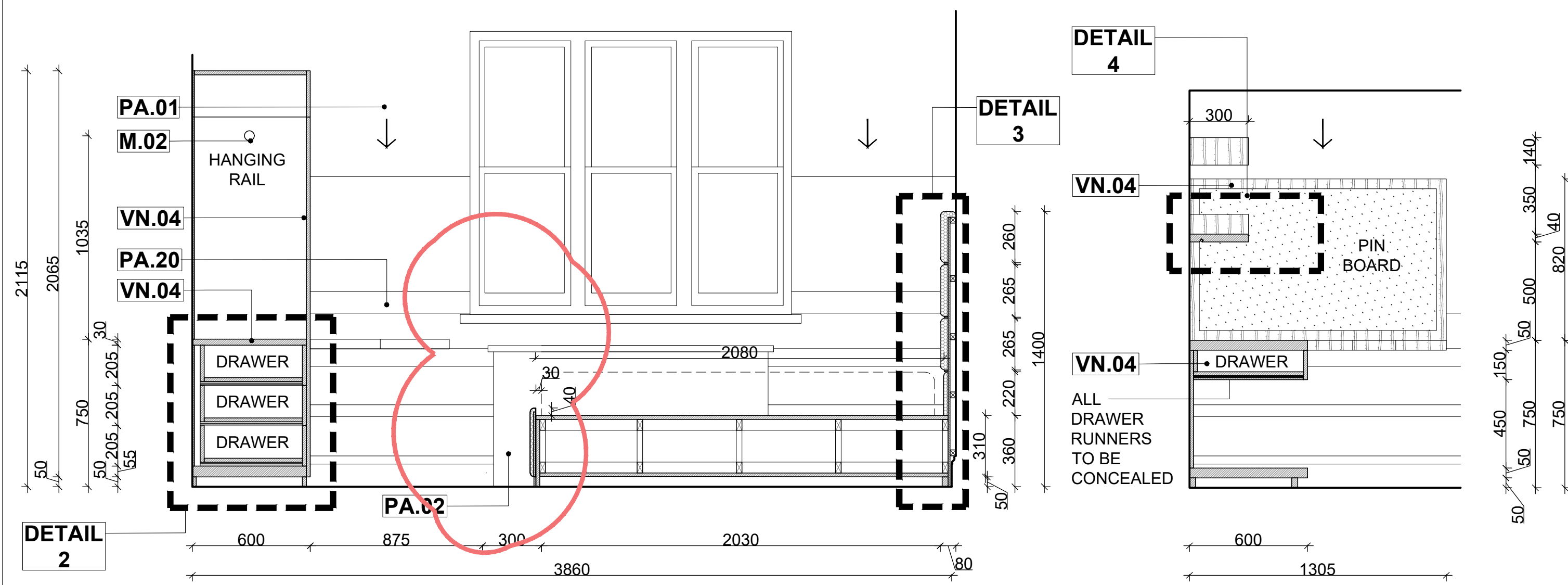
02 SECTION A 1:20 @ A1
