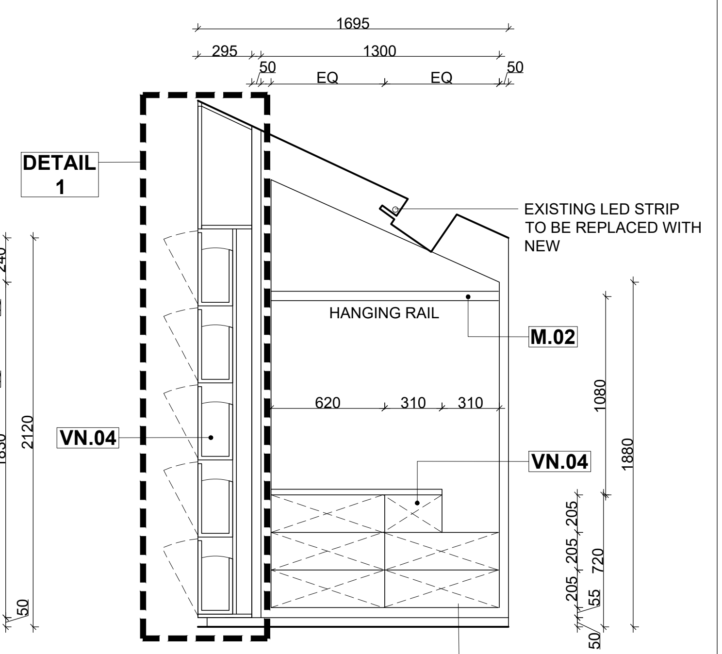
05 ELEVATION A (WITHOUT DOORS) 1:20 @ A1
