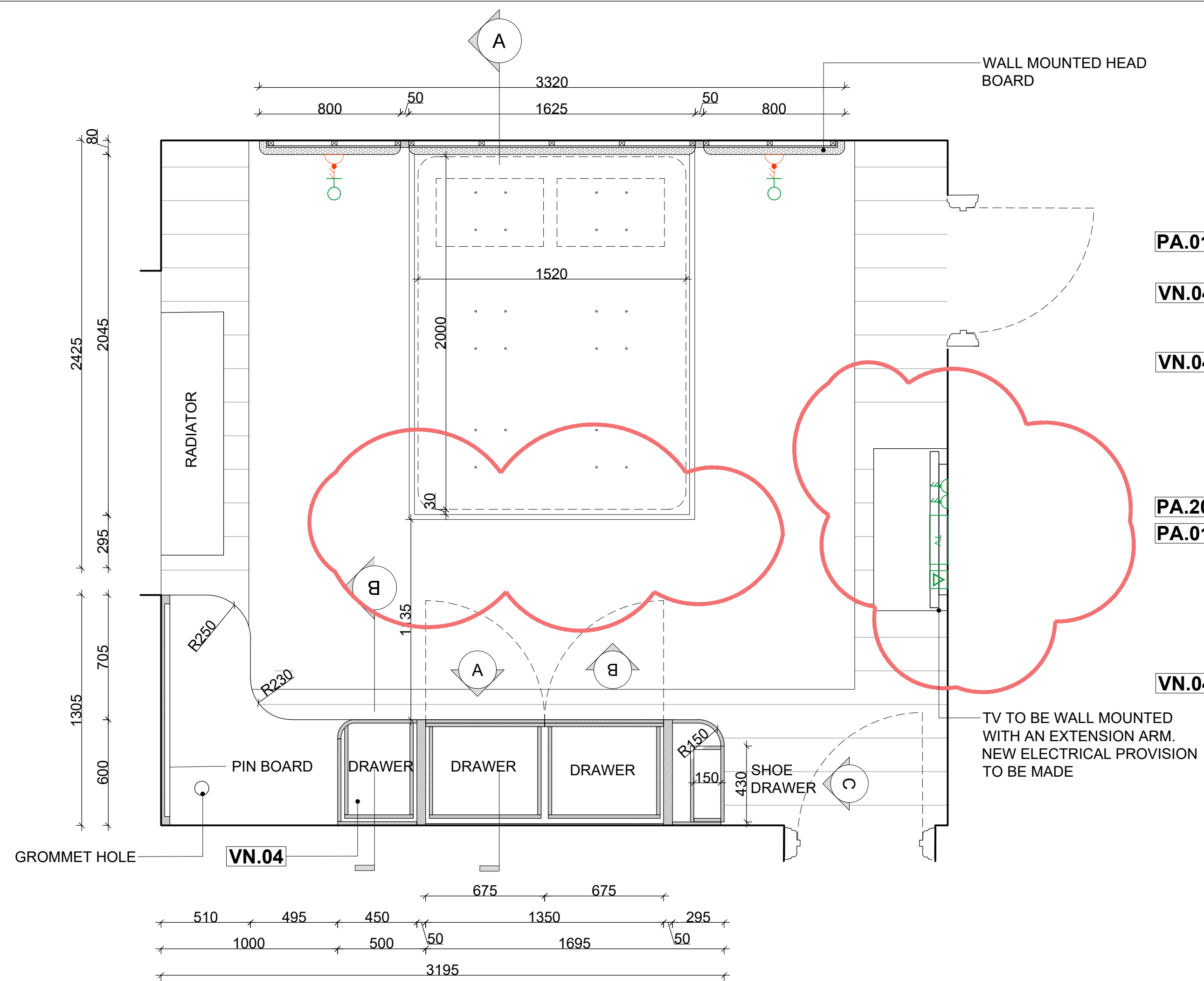
01 PLAN 1:20 @ A1
