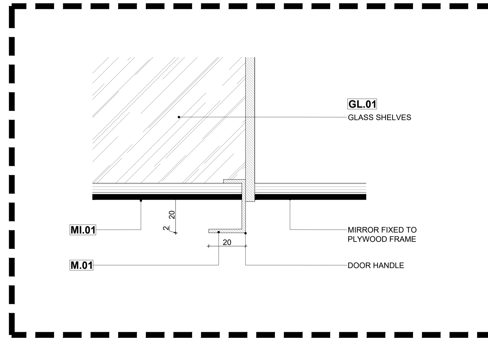
01 DETAIL 3 1:1 @ A1
