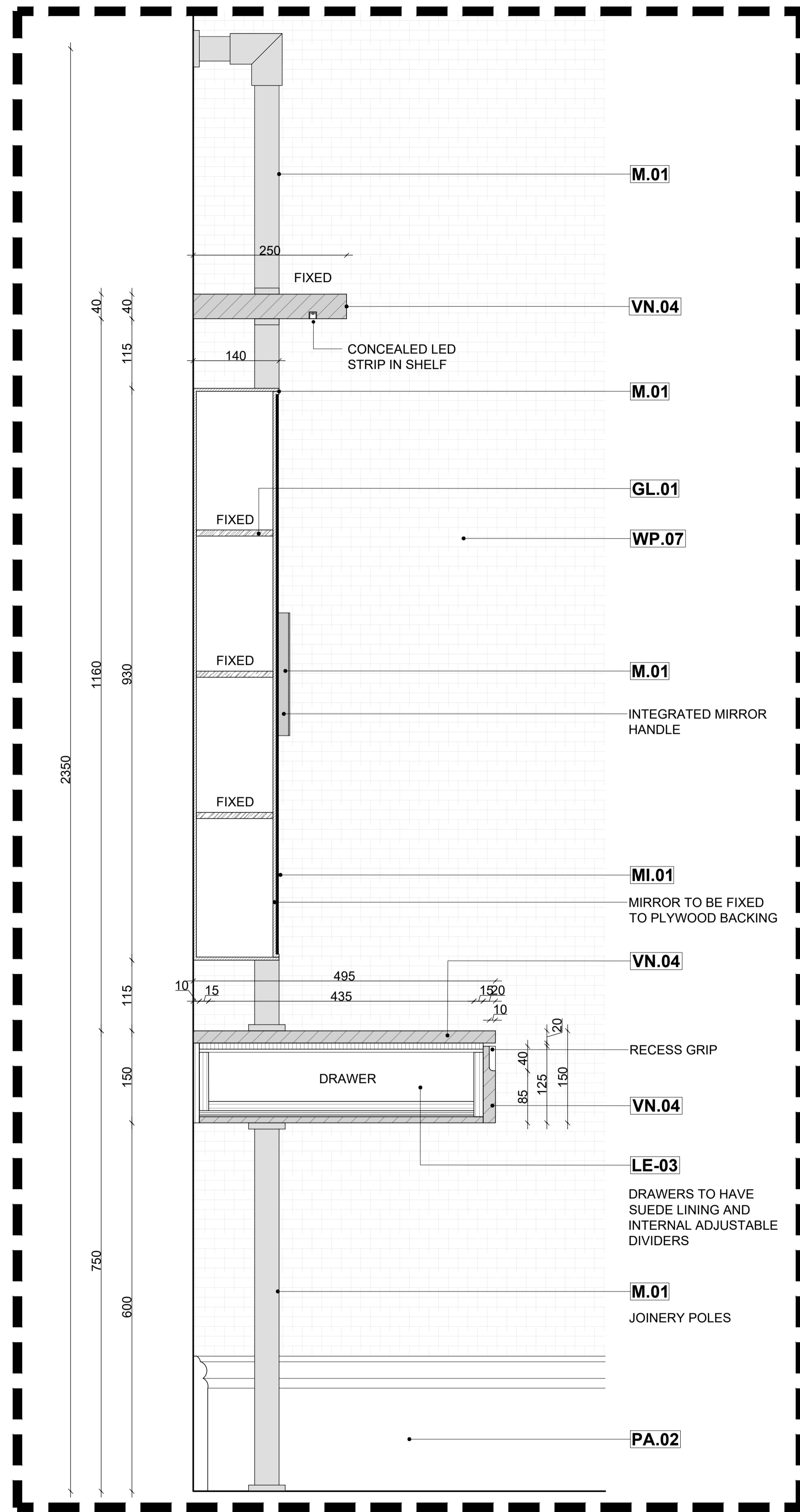
00 DETAIL 3 1:5 @ A1
