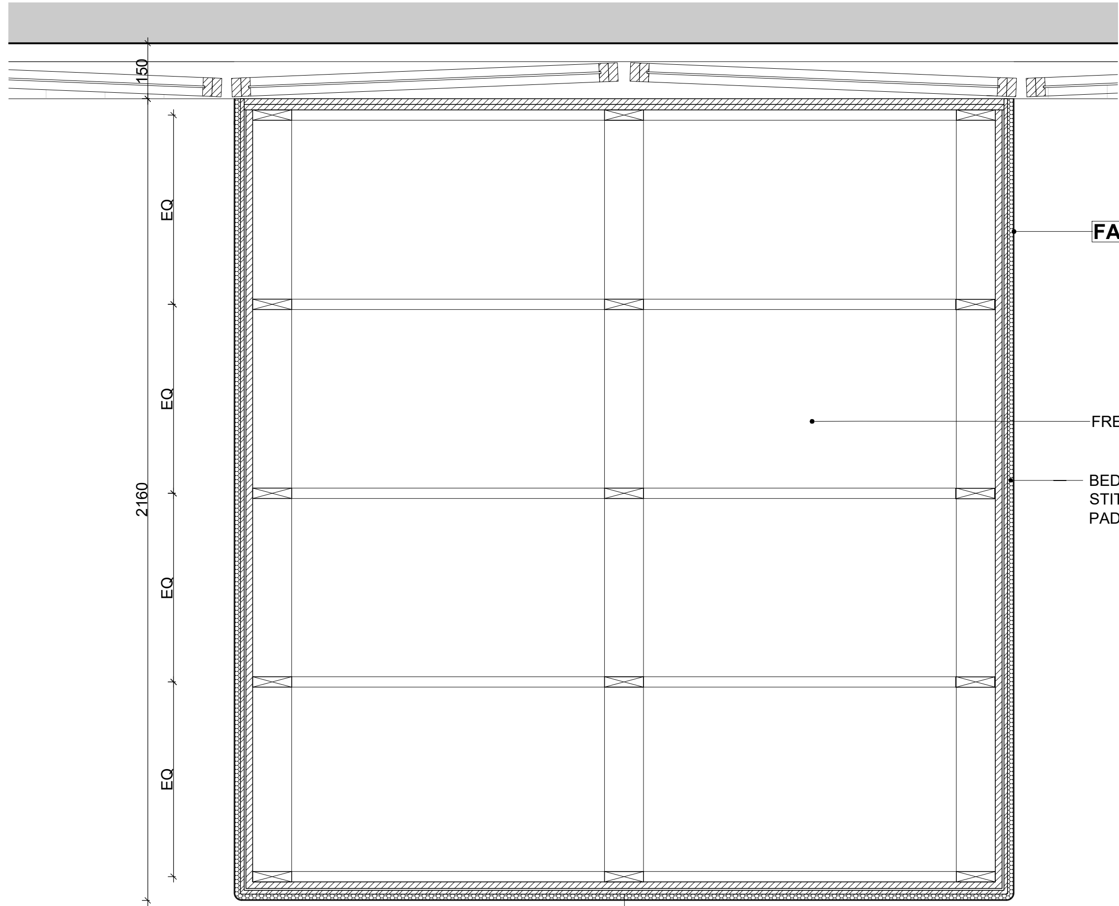
02 PLAN @ B 1:10 @ A1
