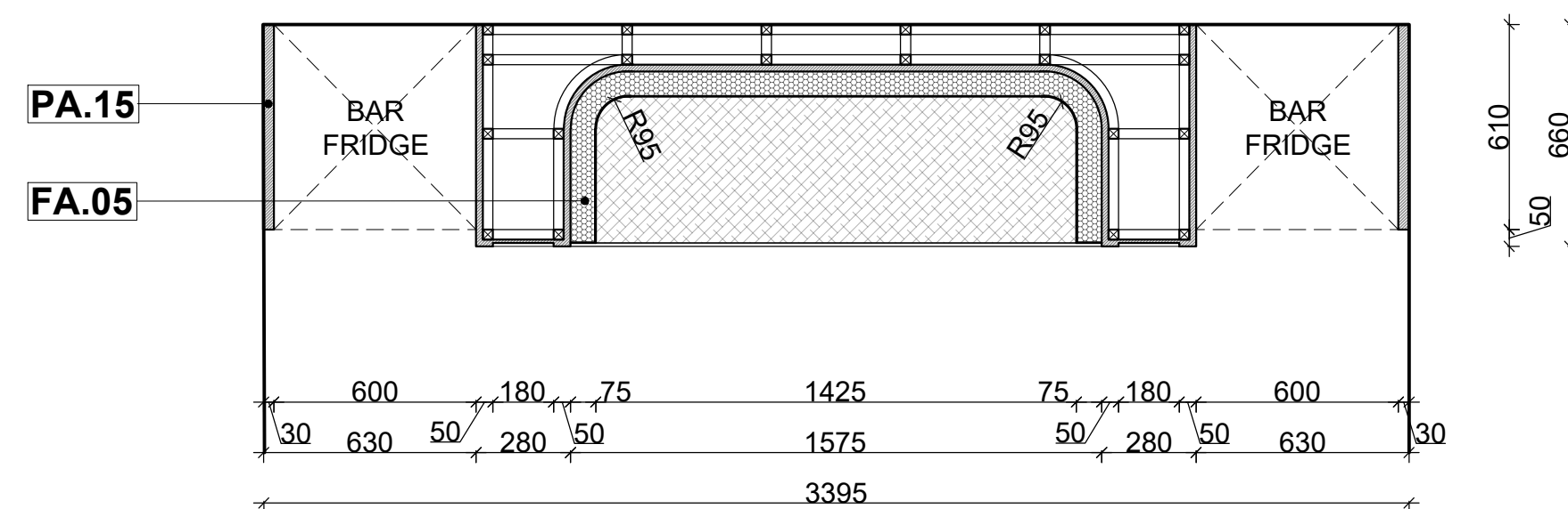
02 PLAN @ B 1:20 @ A1
