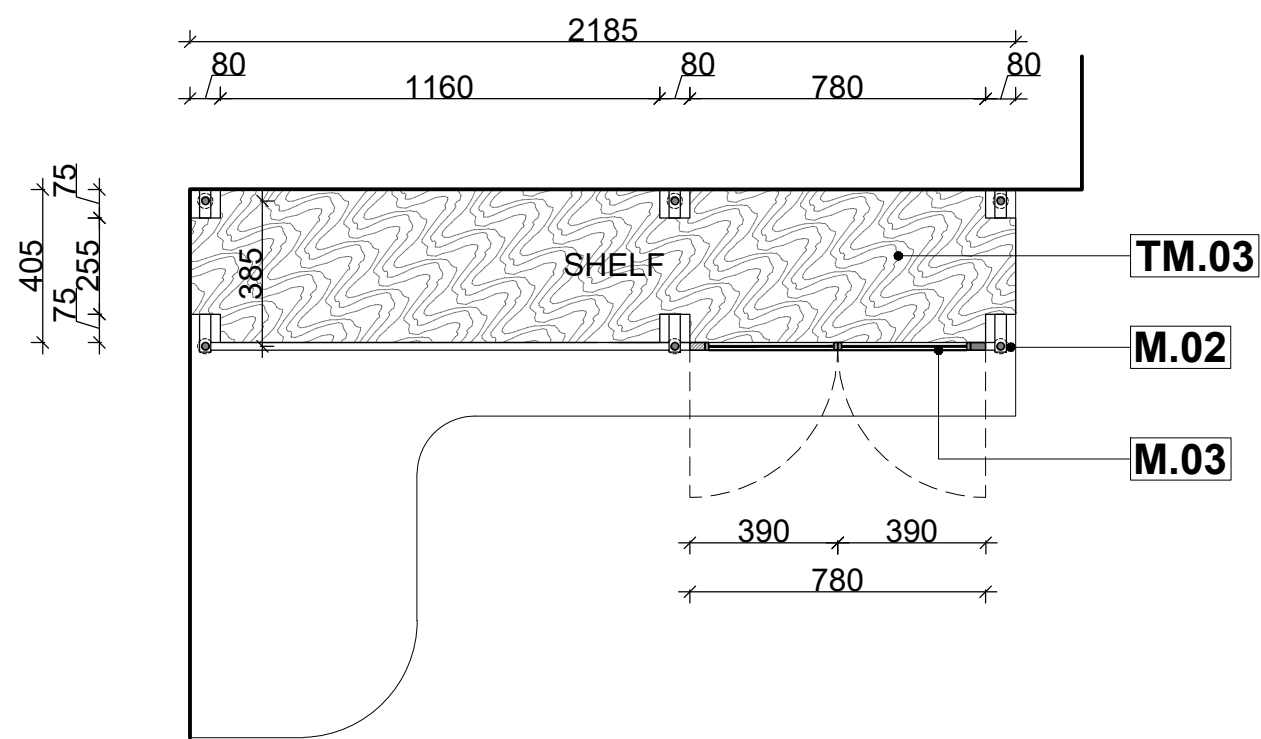
04 PLAN @ C 1:20 @ A1
