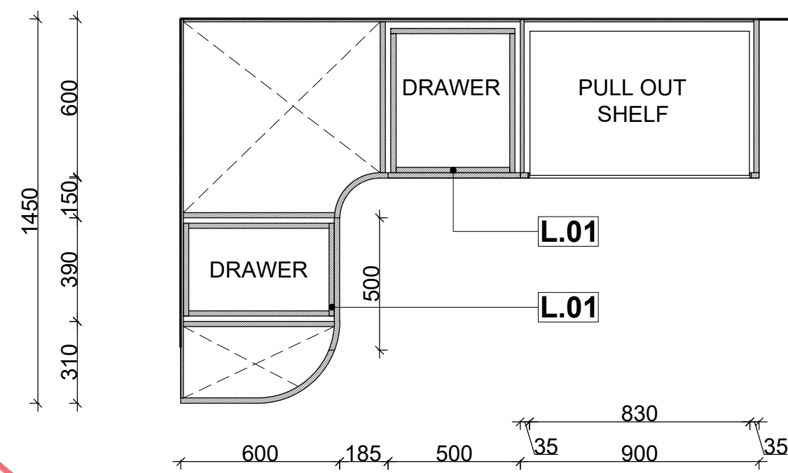
06 PLAN @ E 1:20 @ A1
