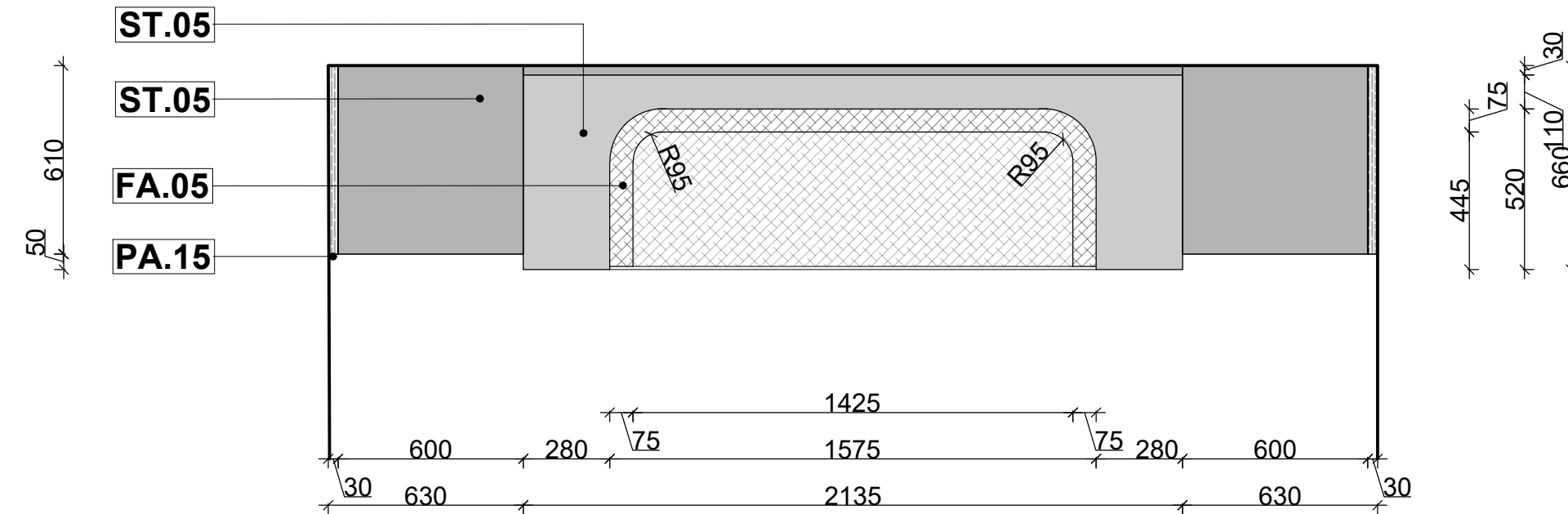
01 PLAN @ A 1:20 @ A1
