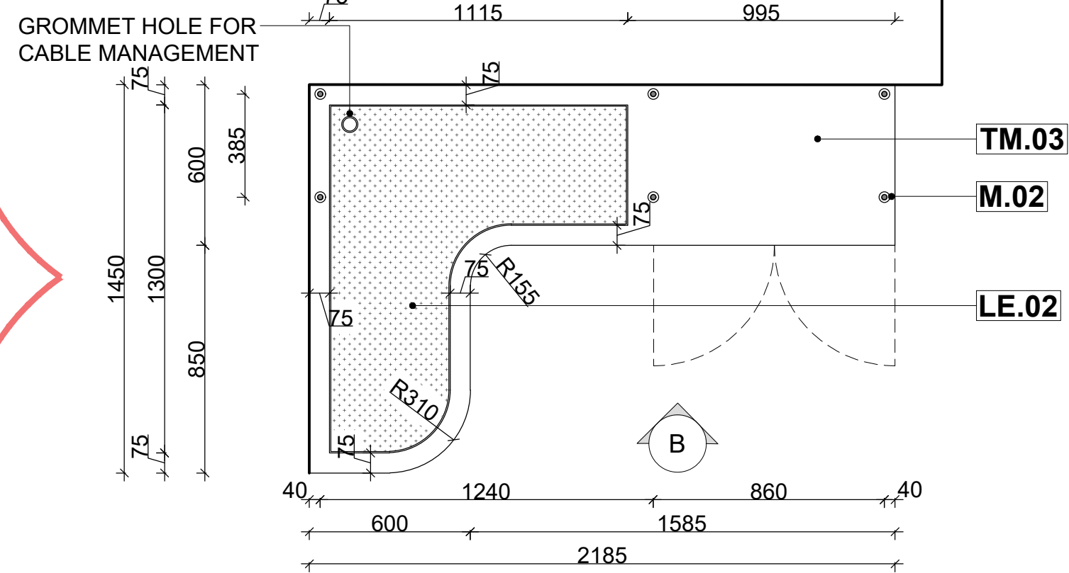
05 PLAN @ D 1:20 @ A1
