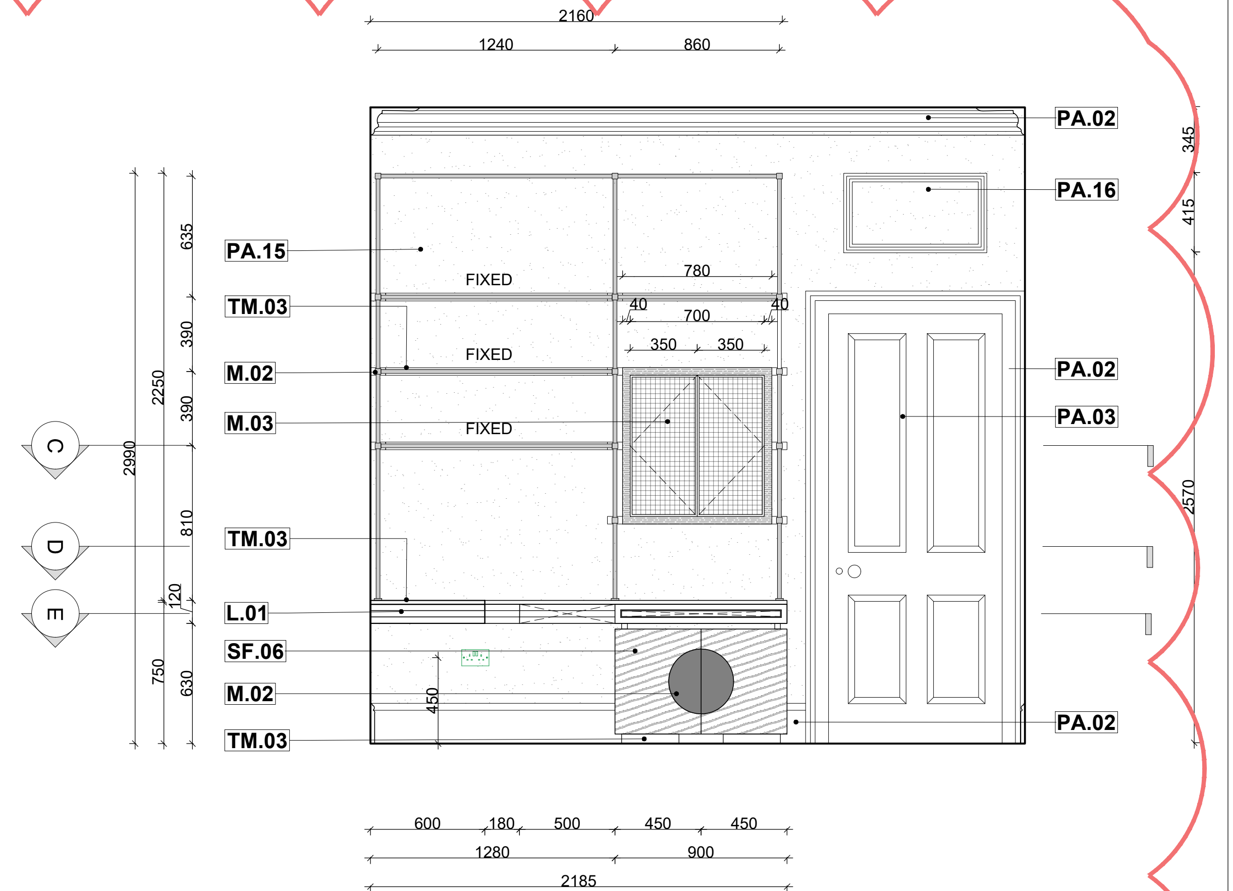
07 ELEVATION B 1:20 @ A1
