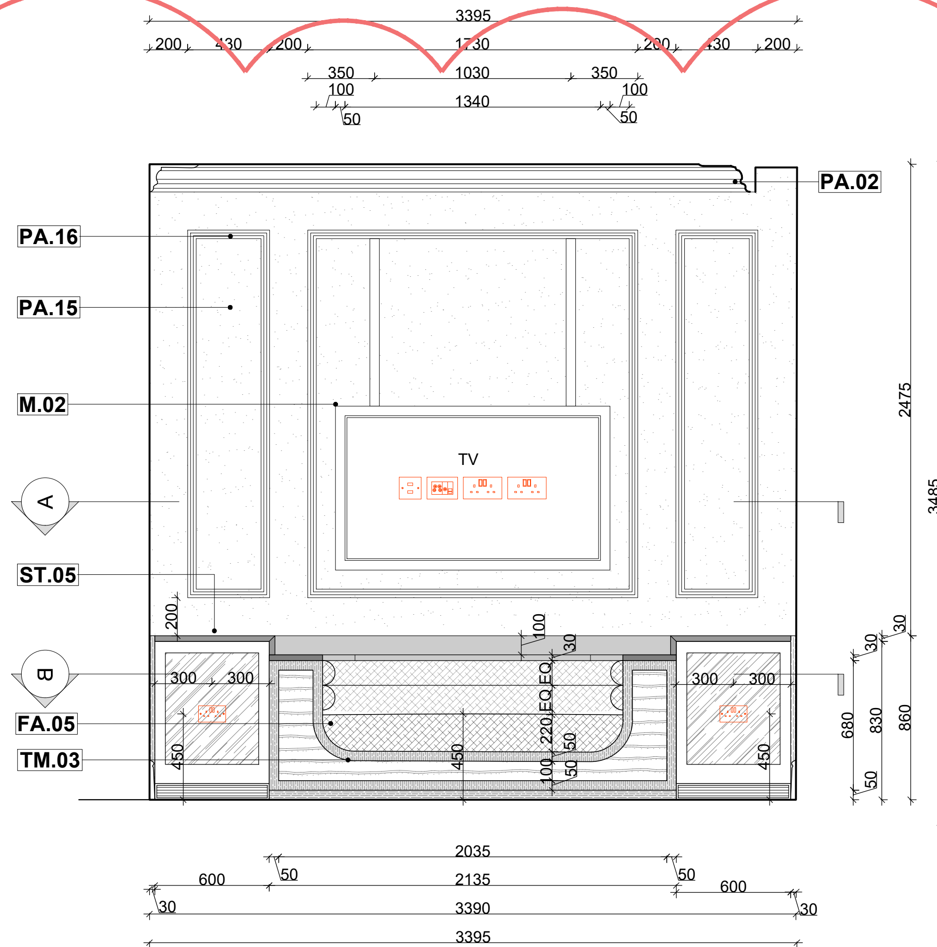
03 ELEVATION A 1:20 @ A1
