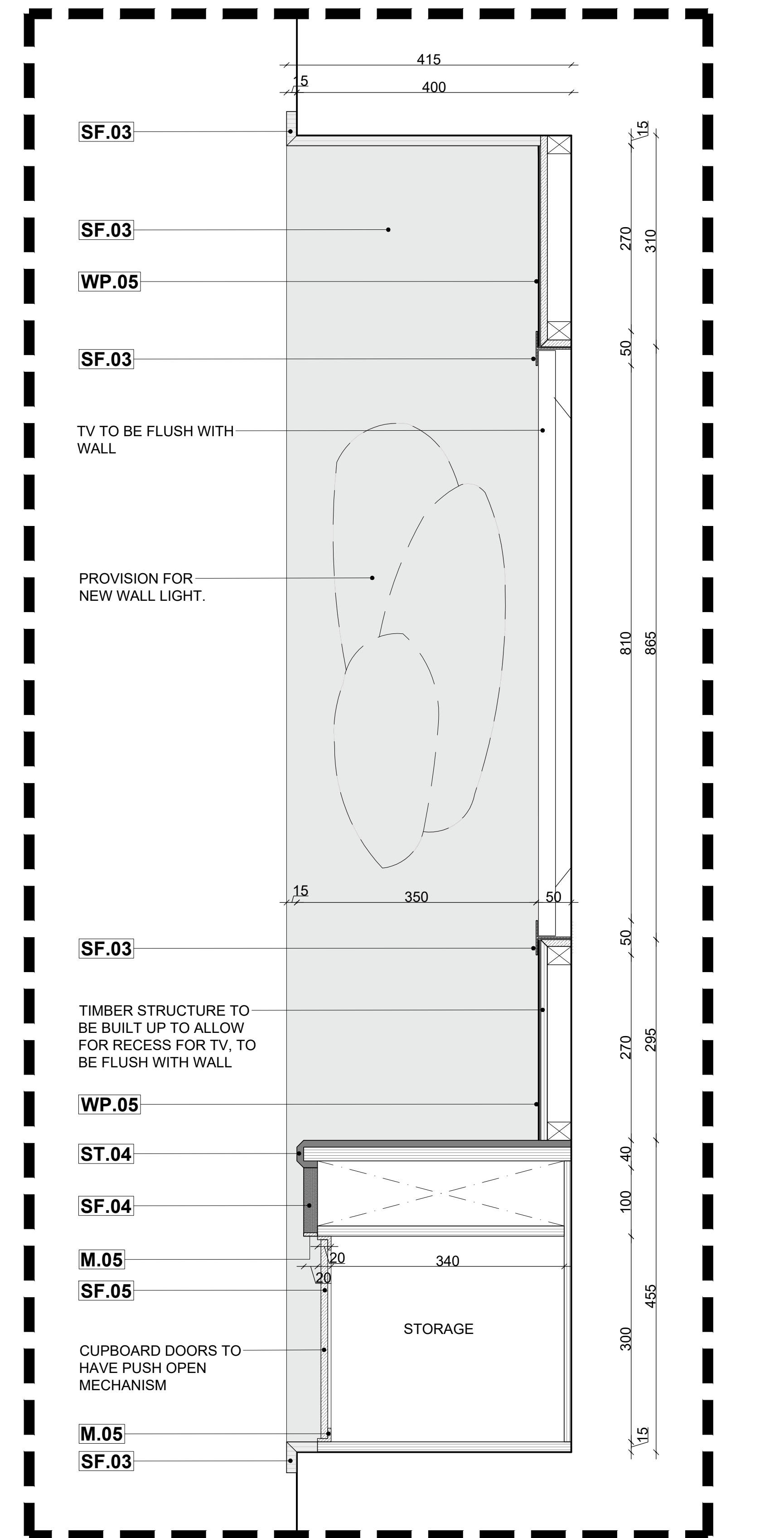
03 DETAIL 1 1:5 @ A1
