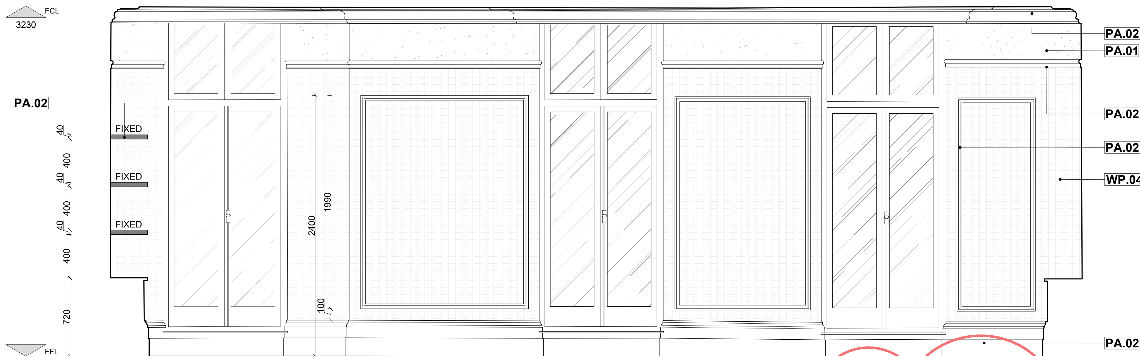
02 ELEVATION C 1:20 @ A1
