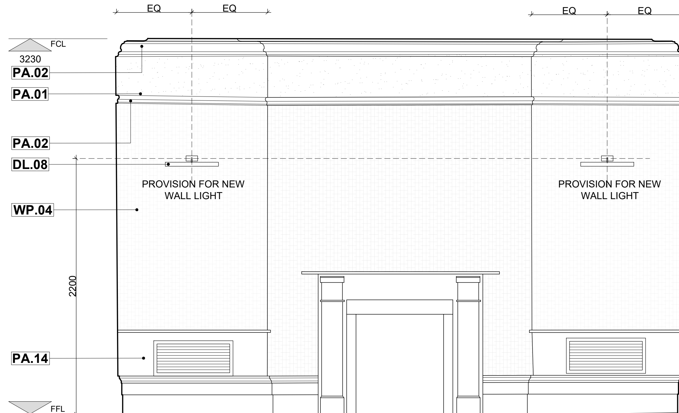
01 ELEVATION B 1:20 @ A1
