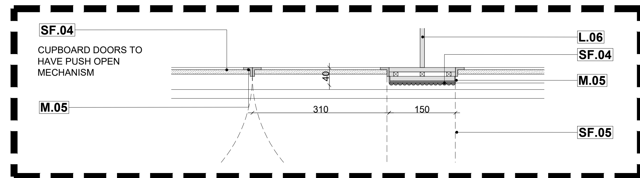
02 ELEVATION C 1:20 @ A1
