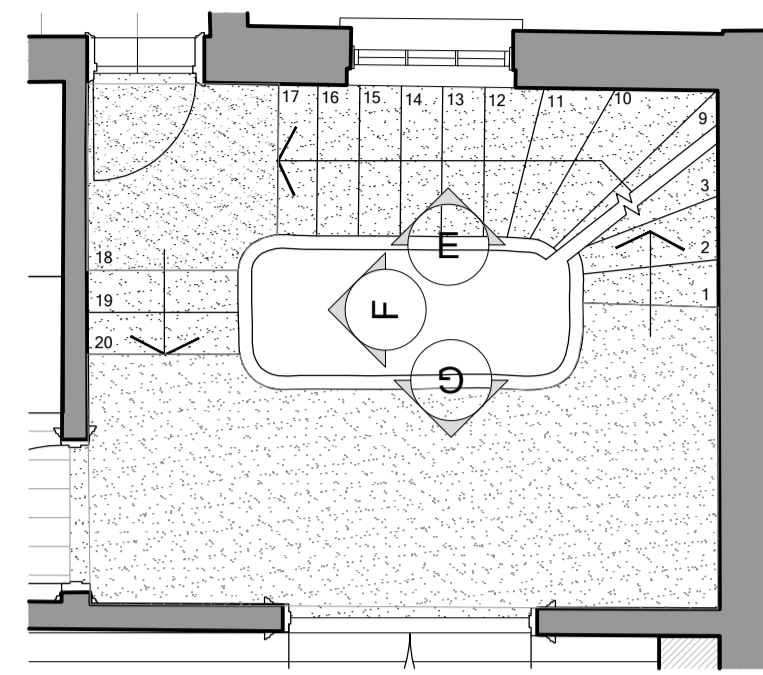
01 KEY PLAN 1:50 @ A1
