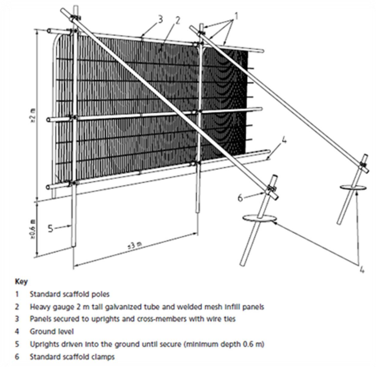
Figure 2: BS5837:2012 - Figure 2, Default specification for protective barriers.
