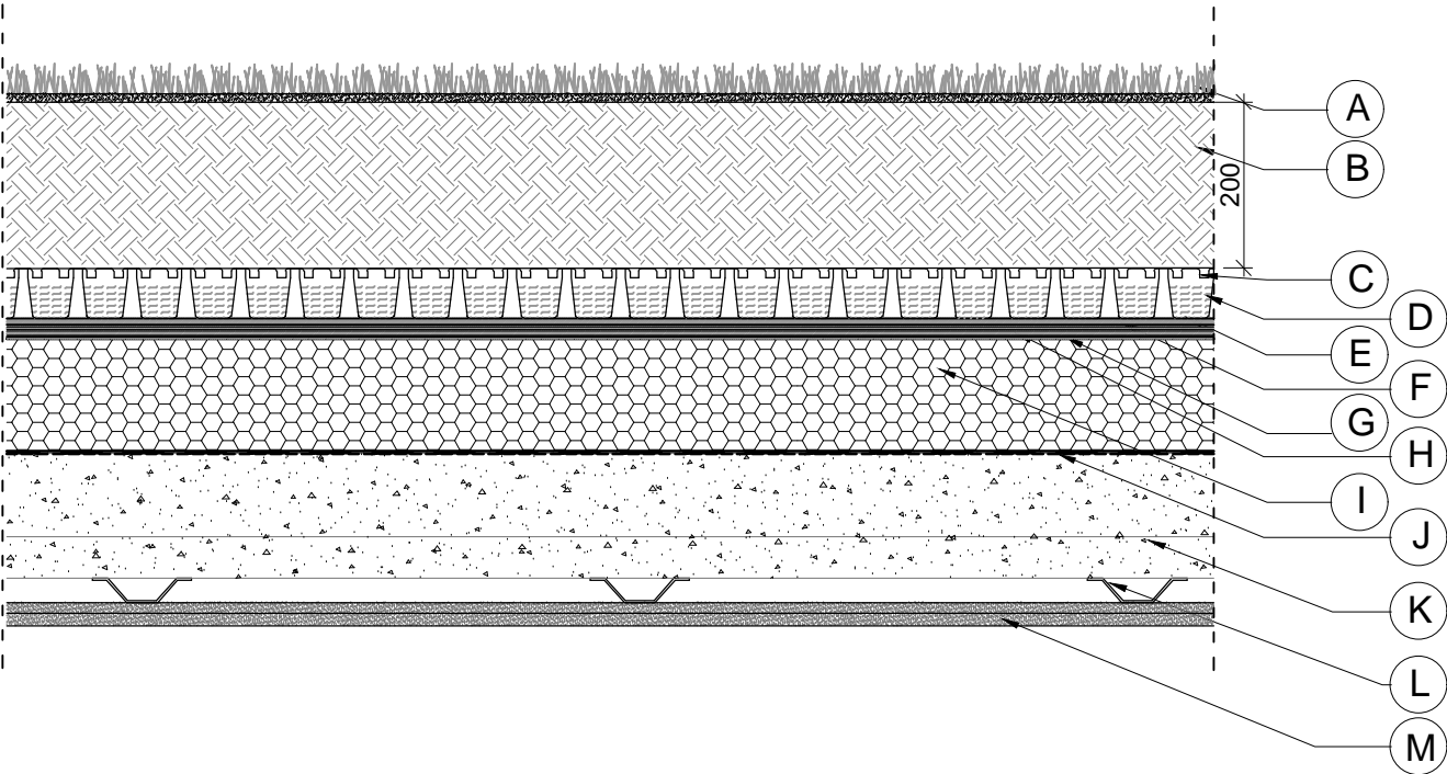
PROPOSED GREEN ROOF BUILD-UP DETAIL
