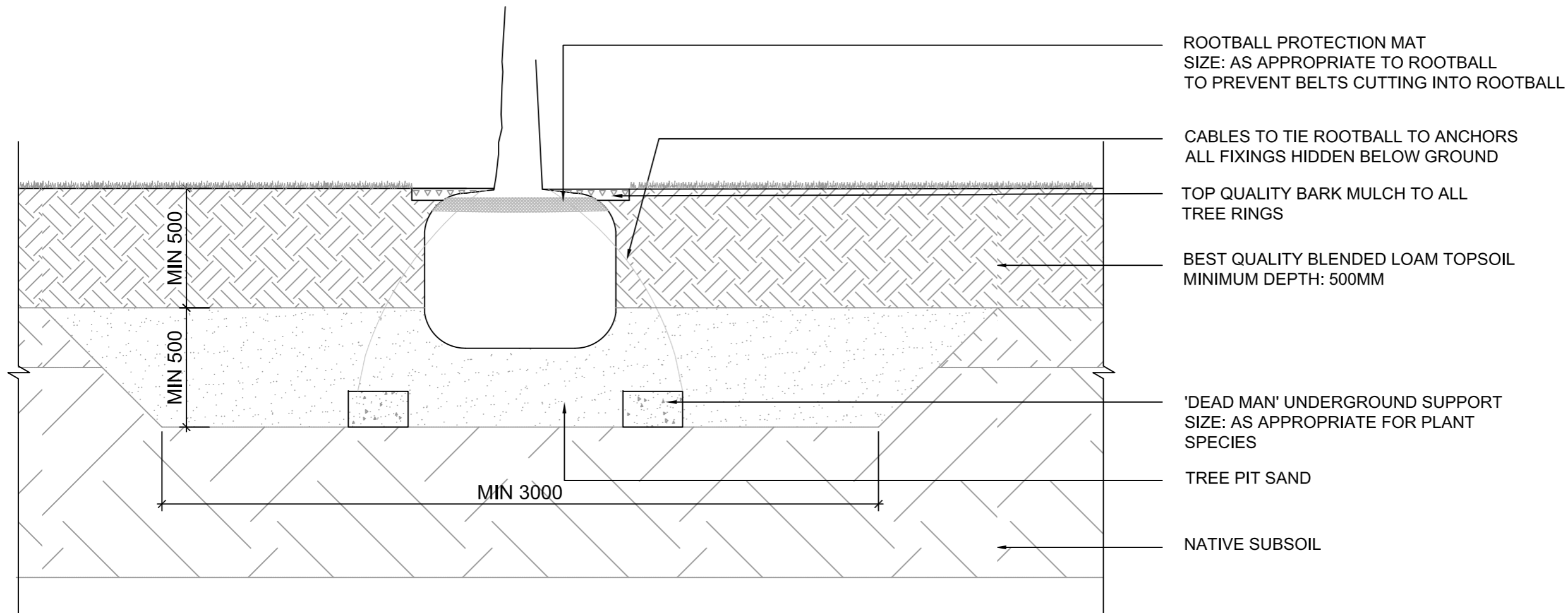
D5 - Proposed Tree Pit in Open Ground
