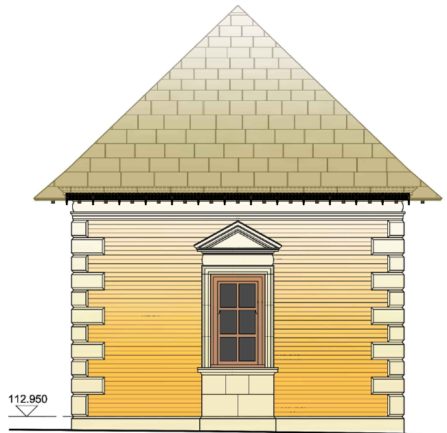
EAST ELEVATION - 1:50
