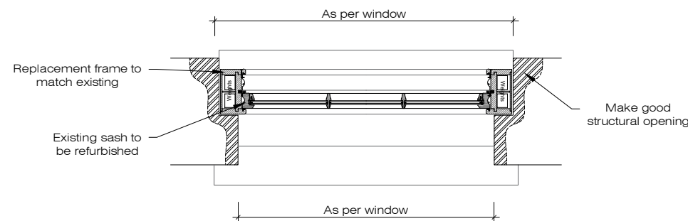
CONSERVATION BOX SASH WINDOW FLUSH REVEAL WITHIN STRUCTURE
