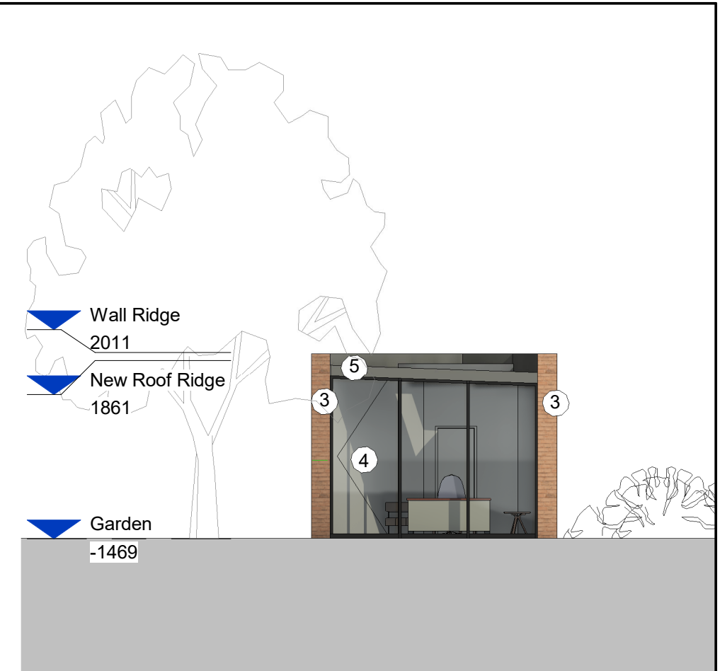
2 GA-ELE-Garden Room 1 : 100
