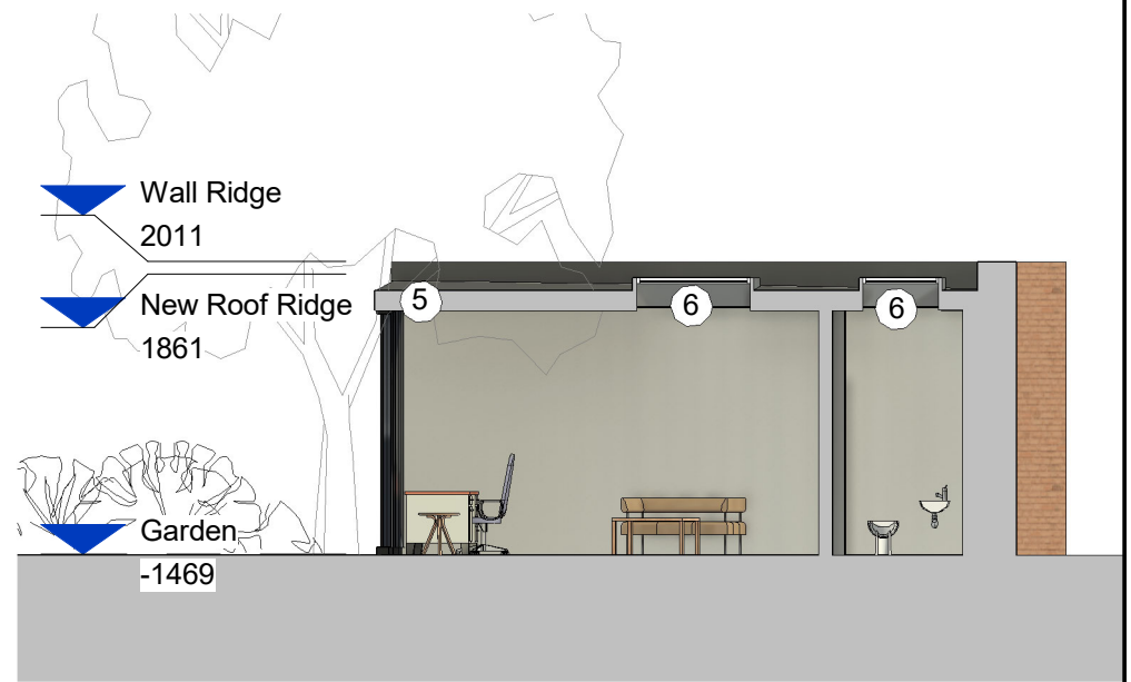
3 GA-SECT-Garden Room 1 : 100
