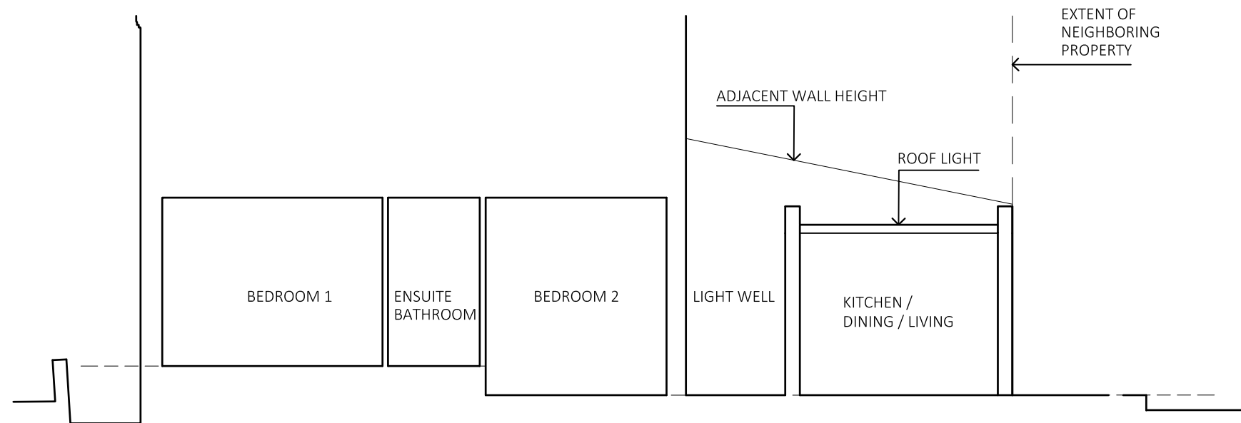
PROPOSED SECTION - A
