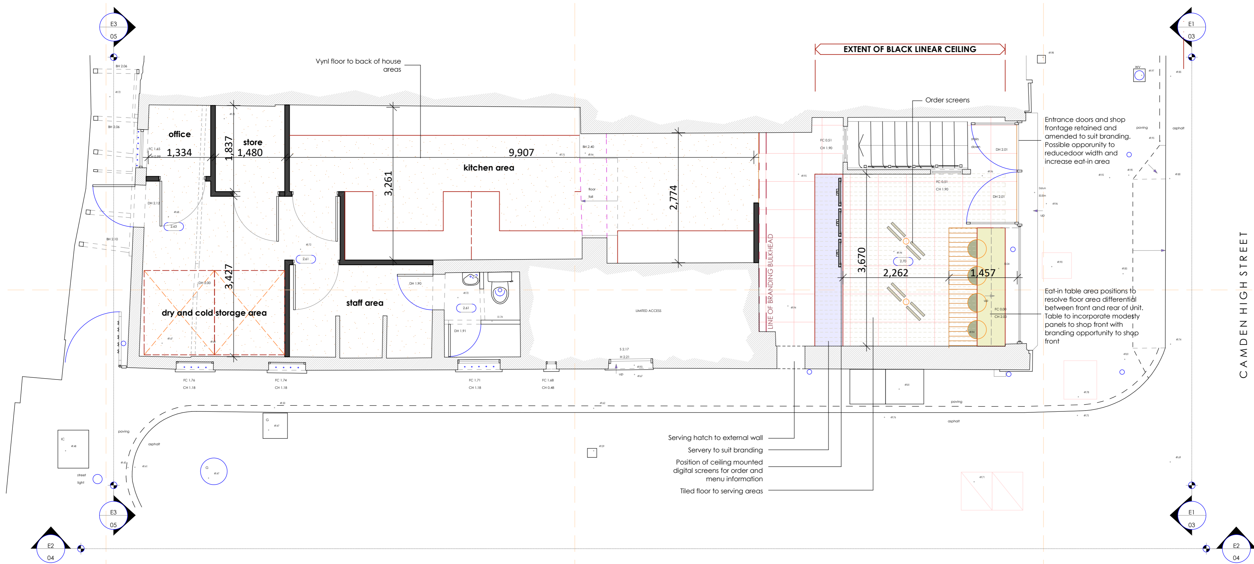
PROPOSED GROUND FLOOR
