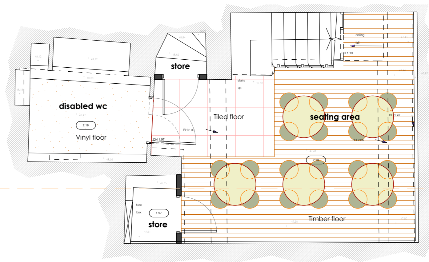
PROPOSED LOWER GROUND FLOOR
